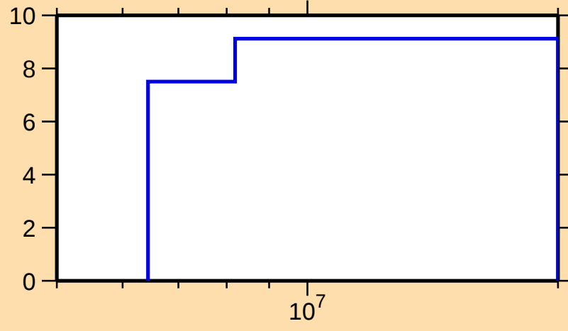
\Delta\sigma/\sigma vs. E for ^{56}\text{Mn}(n,\text{tot.})
