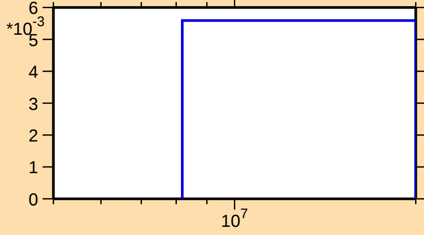
\sigma vs. E for ^{56}\text{Mn}(n,np)
