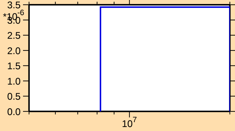
\sigma vs. E for ^{56}\text{Mn}(n,nd)
