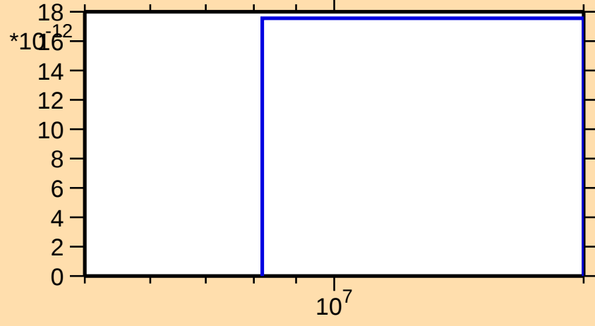
\sigma vs. E for ^{56}\text{Mn}(n,2n\alpha)
