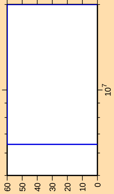
\Delta\sigma/\sigma vs. E for ^{56}\text{Mn}(n,\gamma)
