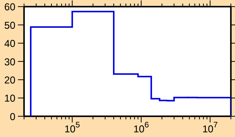
\Delta\sigma/\sigma vs. E for ^{56}\text{Mn}(n,\text{nonel.})
