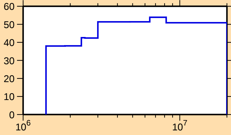
\Delta\sigma/\sigma vs. E for ^{56}\text{Mn}(n,n_1)
