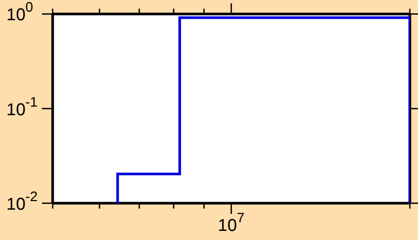
\sigma vs. E for ^{56}\text{Mn}(n,2n)
