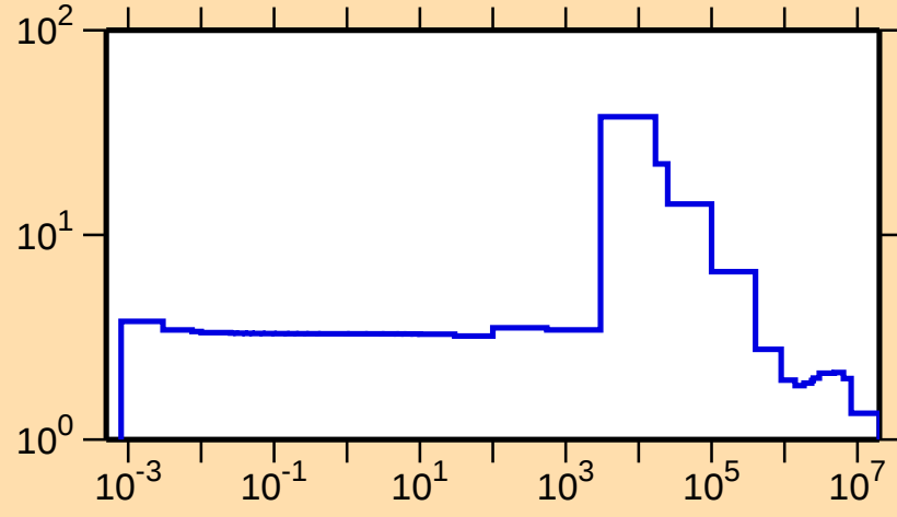
\sigma vs. E for ^{56}\text{Mn}(n,\text{el.})
