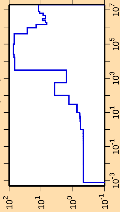
\Delta\sigma/\sigma vs. E for ^{56}\text{Mn}(n,\text{el.})
