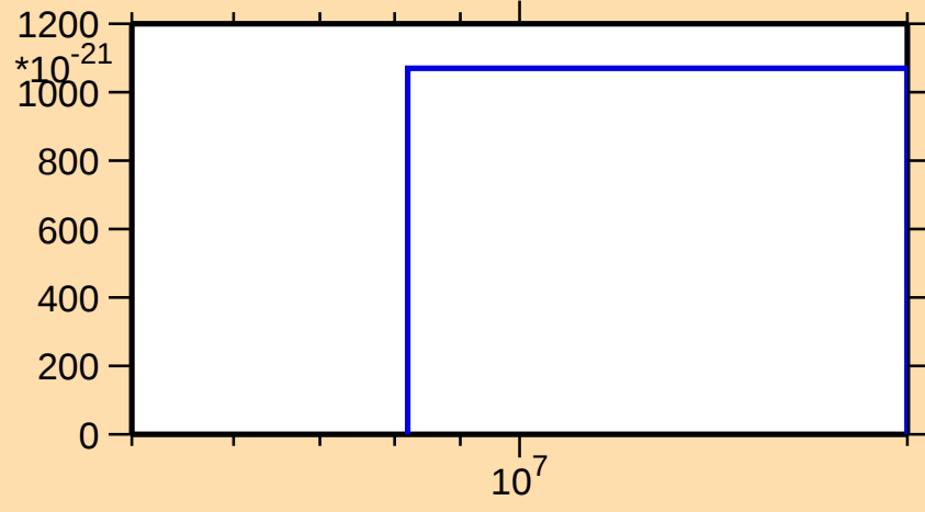
\sigma vs. E for ^{56}\text{Mn}(\text{mt117})
