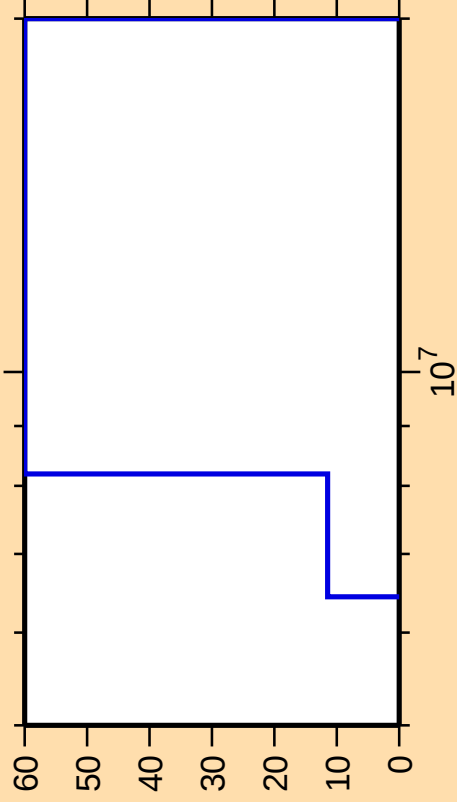
\Delta\sigma/\sigma vs. E for ^{56}\text{Mn}(n,t)
