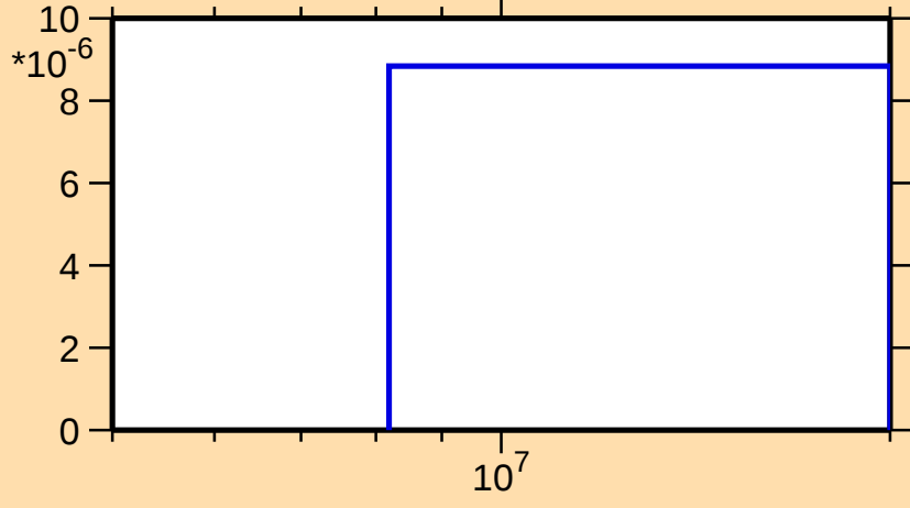
\sigma vs. E for ^{56}\text{Mn}(n,3n)
