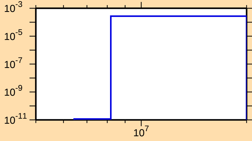
\sigma vs. E for ^{56}\text{Mn}(n,t)
