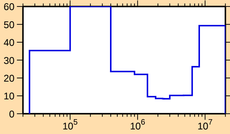
\Delta\sigma/\sigma vs. E for ^{56}\text{Mn}(n,\text{inel.})
