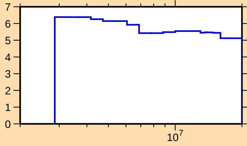
\Delta\sigma/\sigma vs. E for ^{94}\text{Mo}(n,n\text{oncl.})
