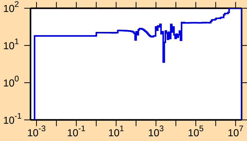
\Delta\sigma/\sigma vs. E for ^{94}\text{Mo}(n,\gamma)
