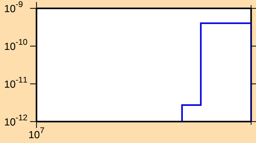
\sigma vs. E for ^{94}\text{Mo}(\text{mt117})
