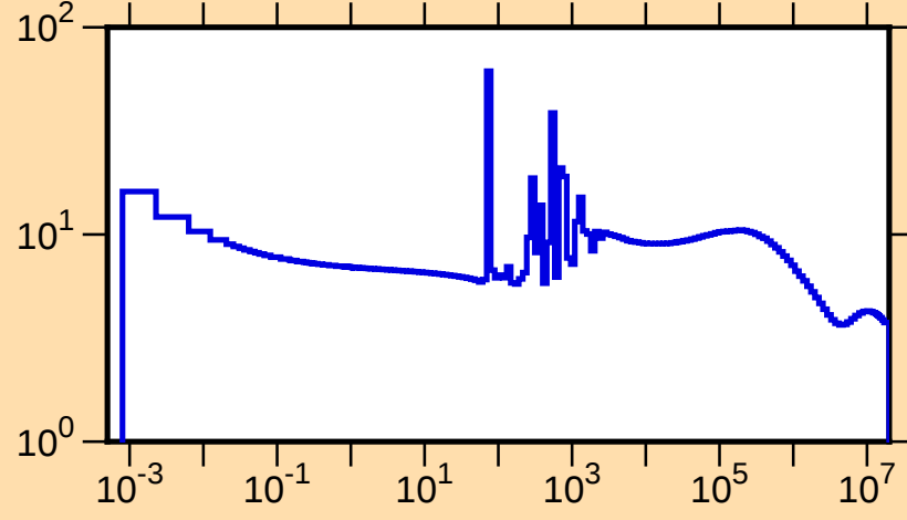
\sigma vs. E for ^{97}\text{Mo}(n,\text{tot.})
