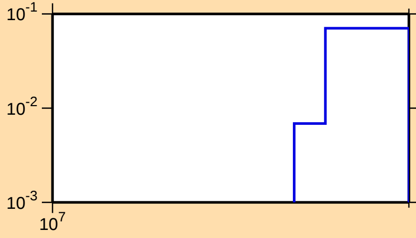
\sigma vs. E for ^{97}\text{Mo}(n,3n)
