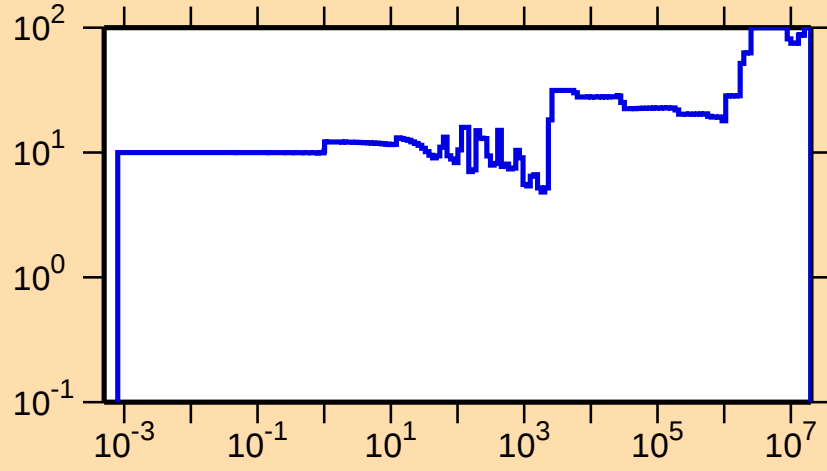
\Delta\sigma/\sigma vs. E for ^{97}\text{Mo}(n,\gamma)
