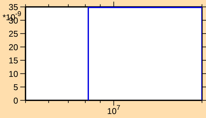
\sigma vs. E for ^{97}\text{Mo}(n,2n\alpha)
