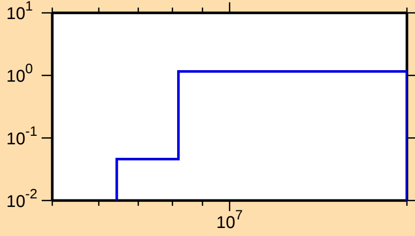
\sigma vs. E for ^{97}\text{Mo}(n,2n)
