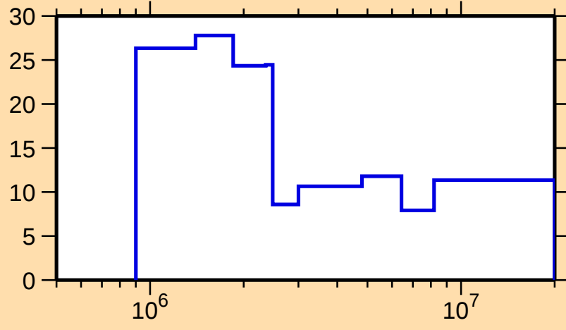
\Delta\sigma/\sigma vs. E for ^{97}\text{Mo}(n,\text{el.})
