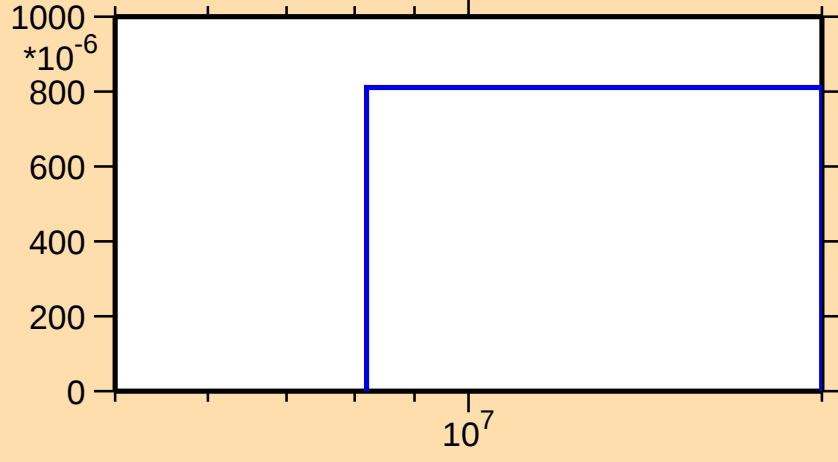
\sigma vs. E for ^{97}\text{Mo}(n,np)
