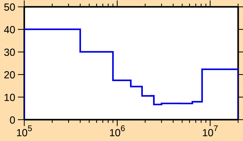
\Delta\sigma/\sigma vs. E for ^{97}\text{Mo}(n,\text{inel.})
