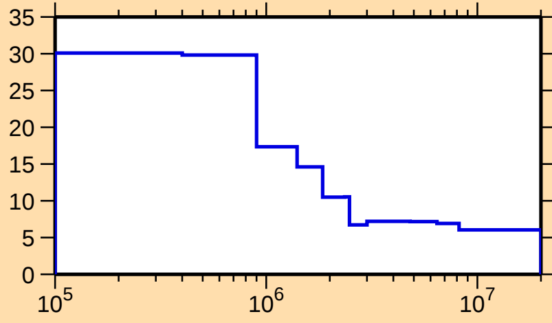
\Delta\sigma/\sigma vs. E for ^{97}\text{Mo}(\text{n,nonel.})
