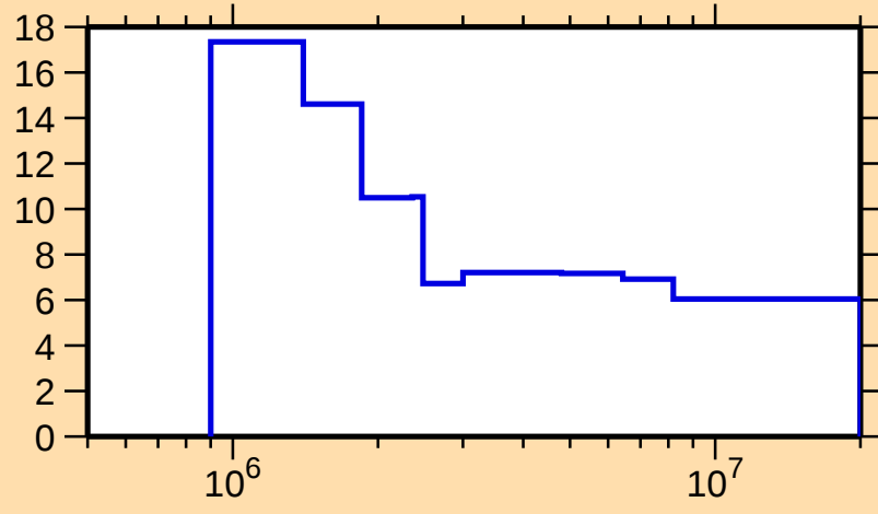
\Delta\sigma/\sigma vs. E for ^{97}\text{Mo}(n,n\text{oncl.})
