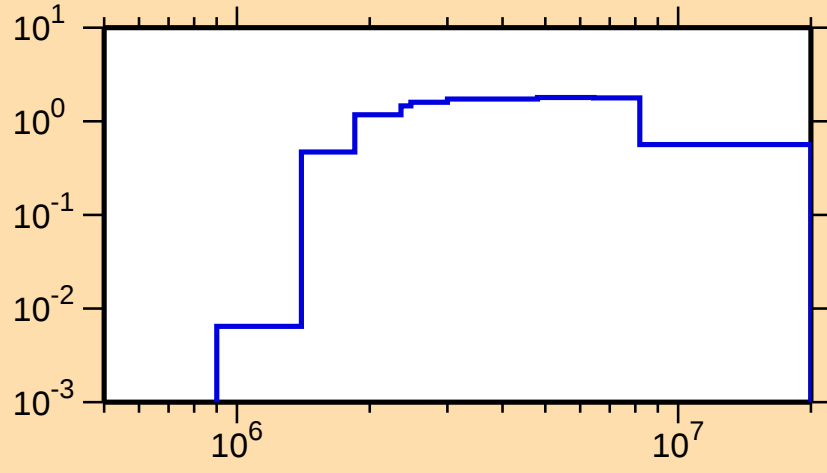
\sigma vs. E for ^{97}\text{Mo}(n,n\text{cont.})
