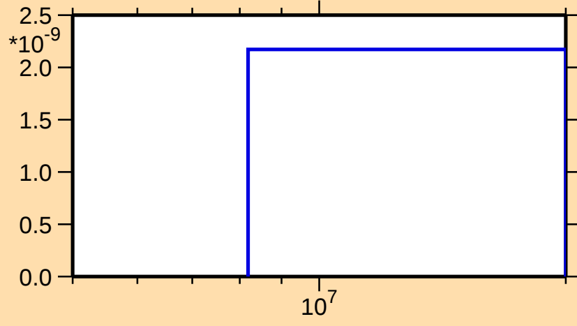
\sigma vs. E for ^{97}\text{Mo}(n,\text{He3})
