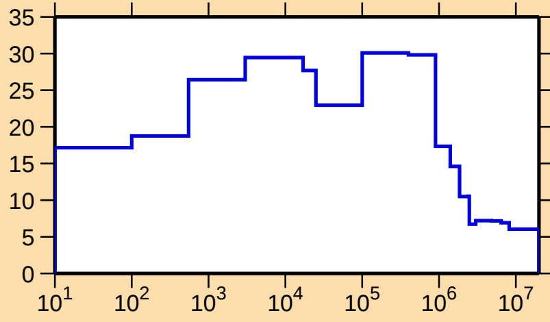
\Delta\sigma/\sigma vs. E for ^{97}\text{Mo}(n,\text{nonel.})
