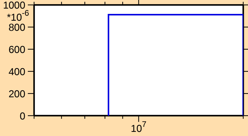
\sigma vs. E for ^{97}\text{Mo}(n,d)
