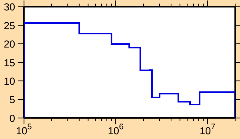
\Delta\sigma/\sigma vs. E for ^{97}\text{Mo}(n,\text{tot.})
