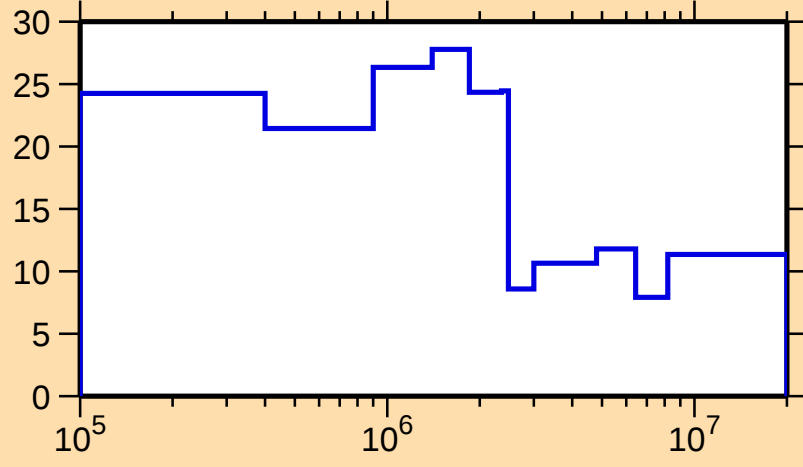
\Delta\sigma/\sigma vs. E for ^{97}\text{Mo}(\text{n,el.})
