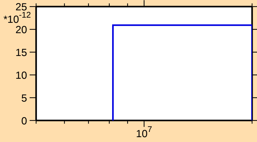
\sigma vs. E for ^{97}\text{Mo}(n,\text{nt})
