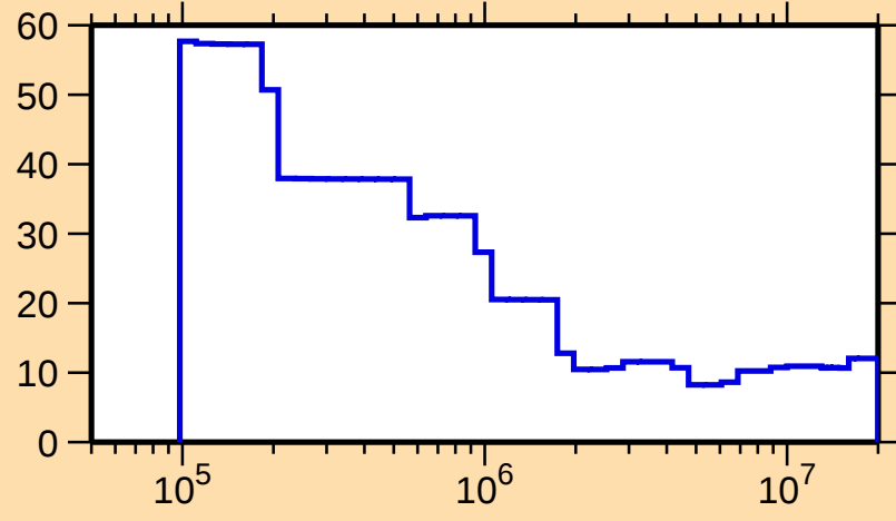
\Delta\sigma/\sigma vs. E for ^{103}\text{Mo}(n,\text{nonel.})
