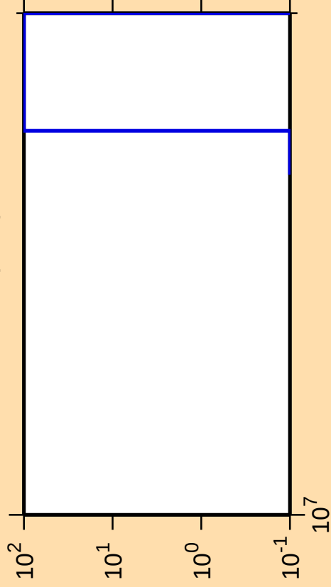
\Delta\sigma/\sigma vs. E for ^{103}\text{Mo}(n,\text{nt})
