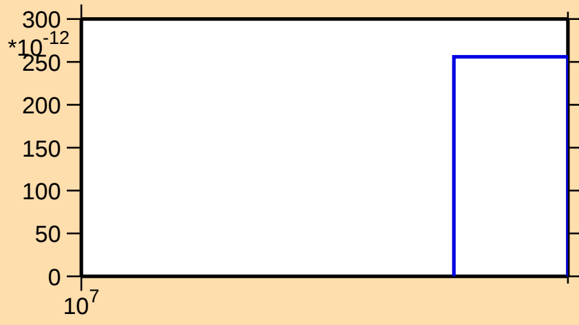
\sigma vs. E for ^{103}\text{Mo}(n,2np)
