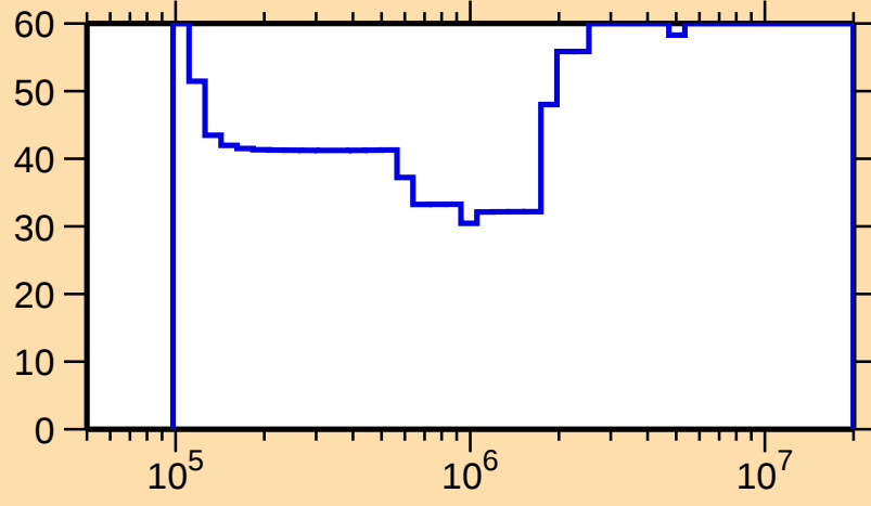
\Delta\sigma/\sigma vs. E for ^{103}\text{Mo}(n,n_1)
