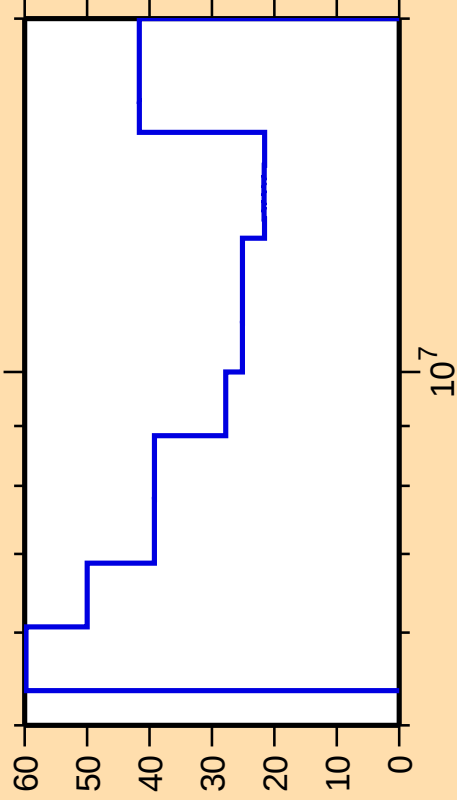
\Delta\sigma/\sigma vs. E for ^{103}\text{Mo}(n,2n)
