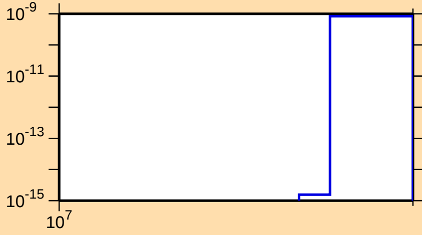
\sigma vs. E for ^{103}\text{Mo}(n,\text{nt})
