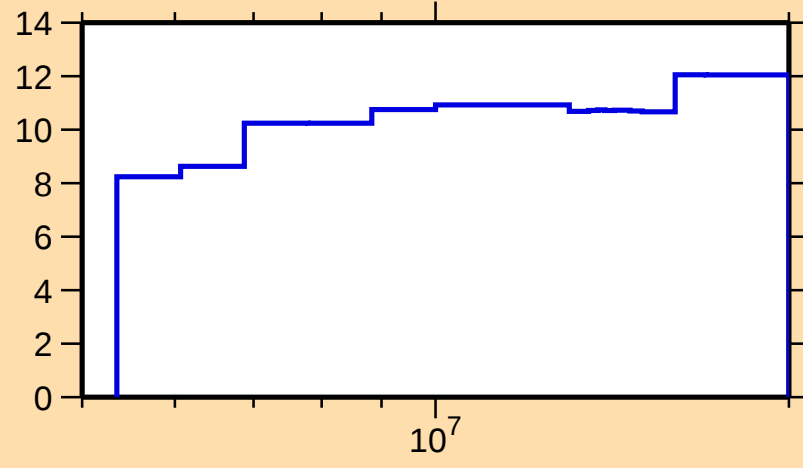
\Delta\sigma/\sigma vs. E for ^{103}\text{Mo}(n,\text{nonel.})
