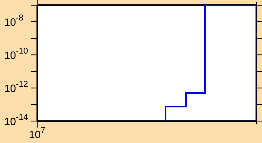
\sigma vs. E for ^{103}\text{Mo}(n,\text{nd})
