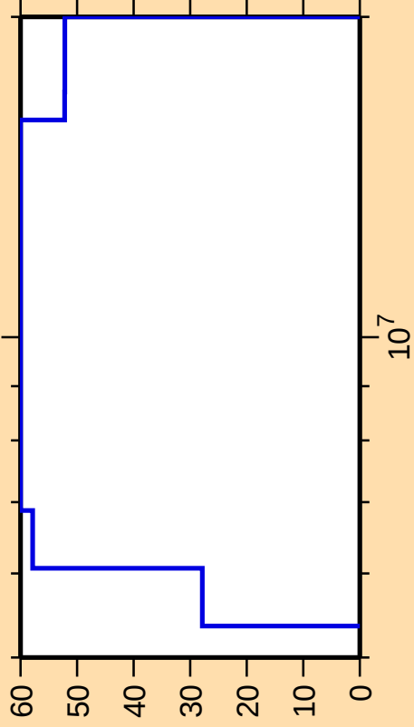
\Delta\sigma/\sigma vs. E for ^{103}\text{Mo}(n,n\text{cont.})
