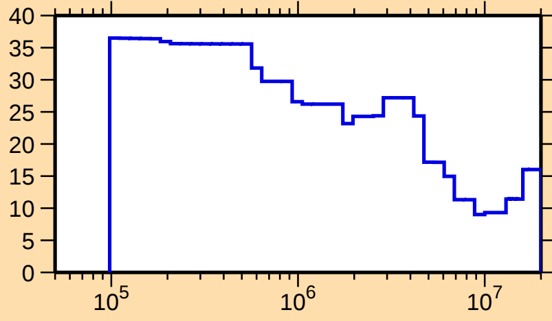
\Delta\sigma/\sigma vs. E for ^{103}\text{Mo}(n,\text{tot.})
