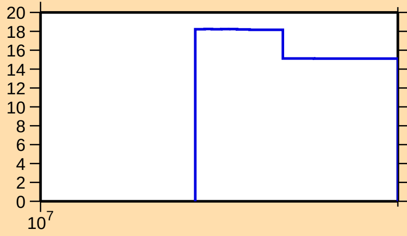
\Delta\sigma/\sigma vs. E for ^{83}\text{Nb}(n,\text{tot.})
