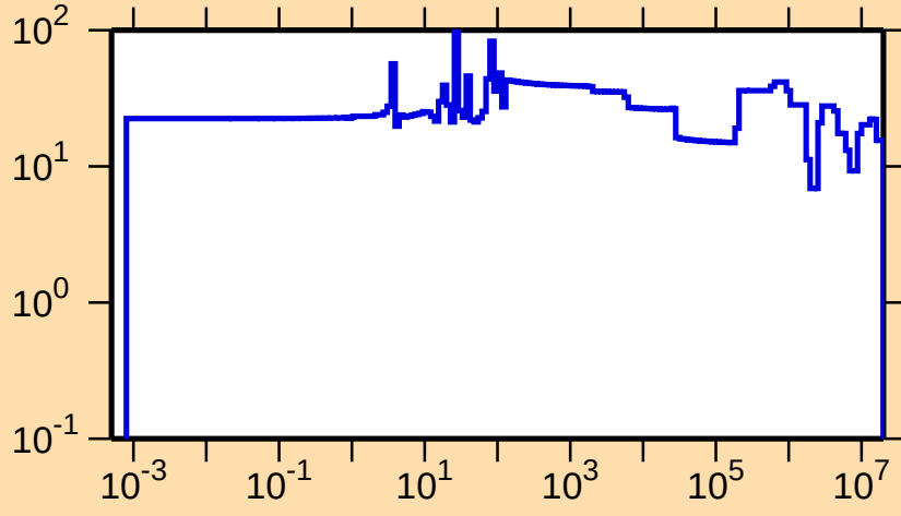
\Delta\sigma/\sigma vs. E for ^{83}\text{Nb}(n,\text{el.})
