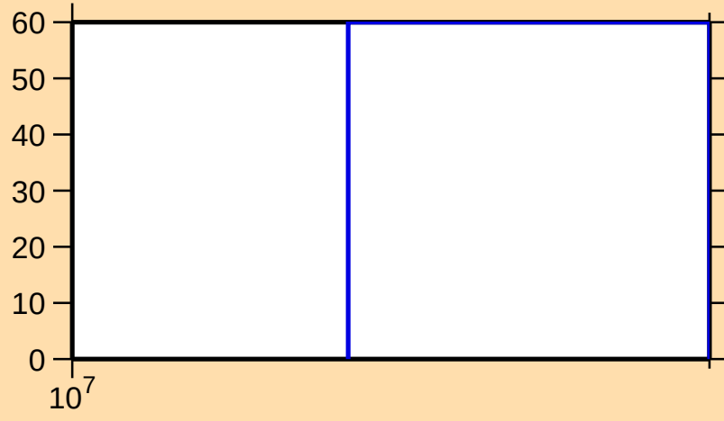
\Delta\sigma/\sigma vs. E for ^{83}\text{Nb}(n,2n)
