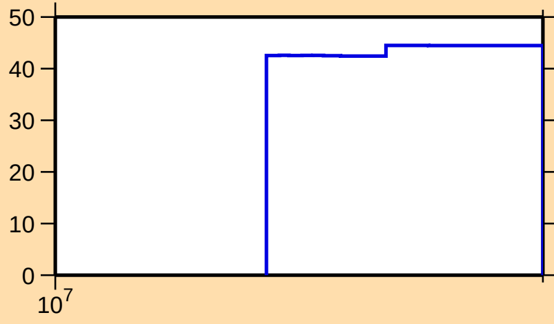
\Delta\sigma/\sigma vs. E for ^{83}\text{Nb}(n,\text{inel.})
