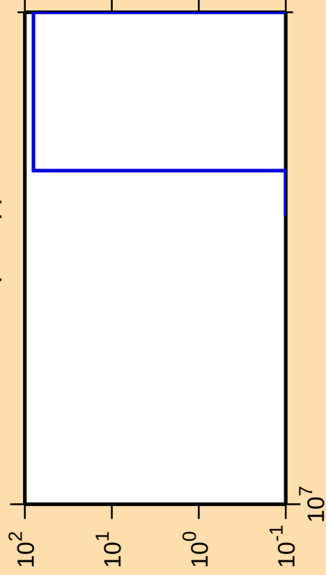
\Delta\sigma/\sigma vs. E for ^{83}\text{Nb}(n,2np)
