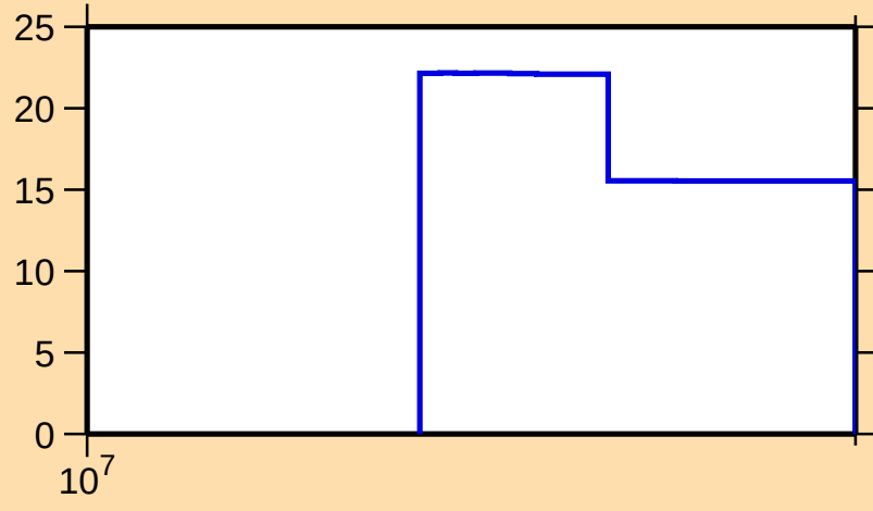
\Delta\sigma/\sigma vs. E for ^{83}\text{Nb}(n,\text{el.})
