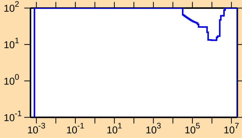
\Delta\sigma/\sigma vs. E for ^{83}\text{Nb}(n,p)
