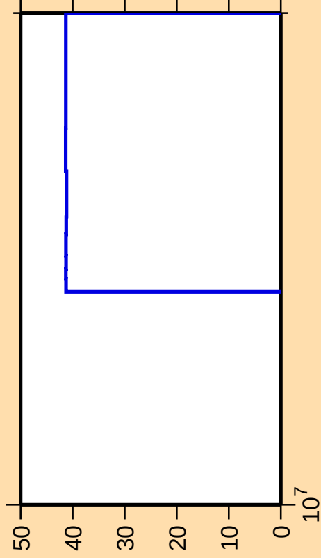
\Delta\sigma/\sigma vs. E for ^{83}\text{Nb}(n,n_1)
