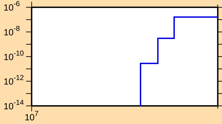
\sigma vs. E for ^{83}\text{Nb}(n,\text{nd})
