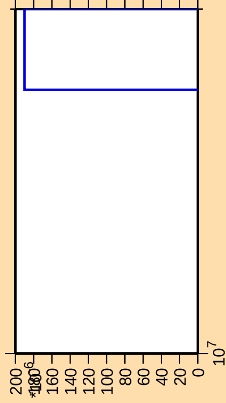
\Delta\sigma/\sigma vs. E for ^{83}\text{Nb}(n,nt)
