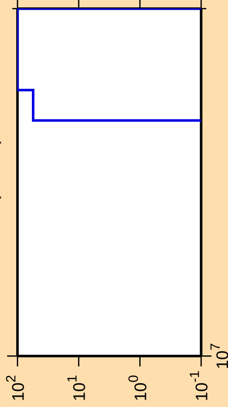
\Delta\sigma/\sigma vs. E for ^{83}\text{Nb}(\text{mt } 34)
