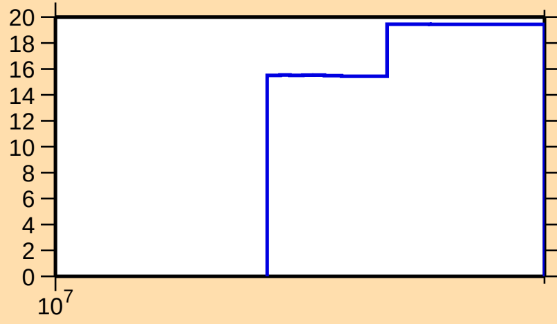
\Delta\sigma/\sigma vs. E for ^{83}\text{Nb}(n,\text{nonel.})
