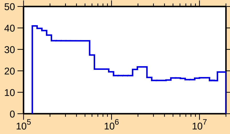
\Delta\sigma/\sigma vs. E for ^{83}\text{Nb}(n,\text{nonel.})
