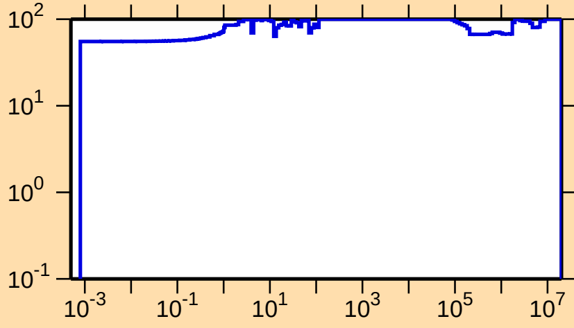
\Delta\sigma/\sigma vs. E for ^{83}\text{Nb}(n,\gamma)
