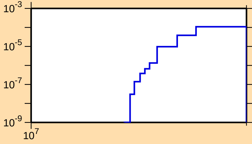
\sigma vs. E for ^{83}\text{Nb}(n,2n)
