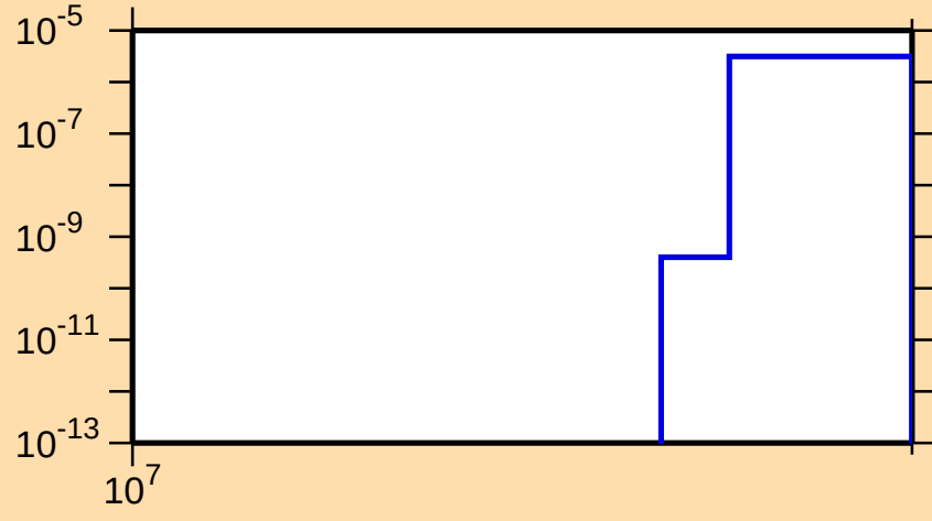
\sigma vs. E for ^{83}\text{Nb}(n,2np)
