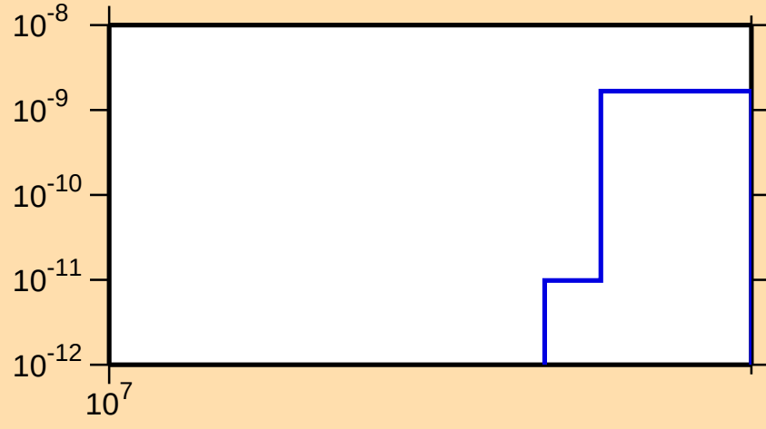
\sigma vs. E for ^{83}\text{Nb}(\text{mt } 34)
