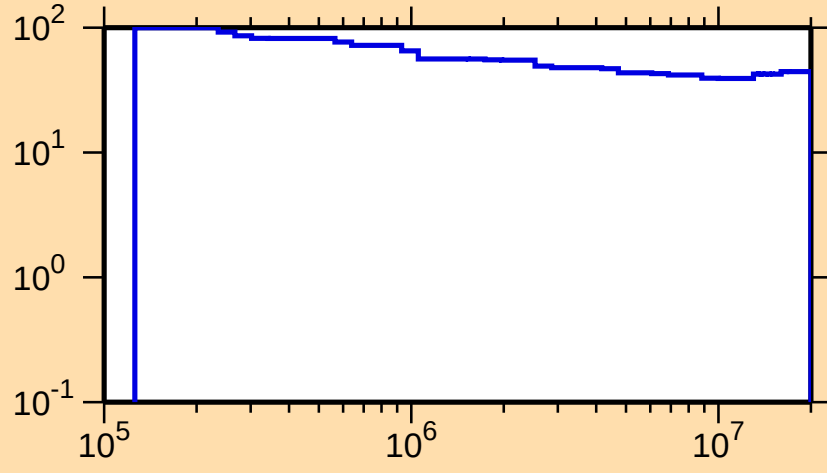
\Delta\sigma/\sigma vs. E for ^{83}\text{Nb}(n,\text{inel.})
