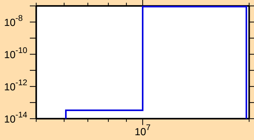
\sigma vs. E for ^{83}\text{Nb}(\text{mt117})
