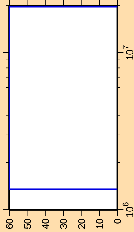
\Delta\sigma/\sigma vs. E for ^{83}\text{Nb}(n,np)
