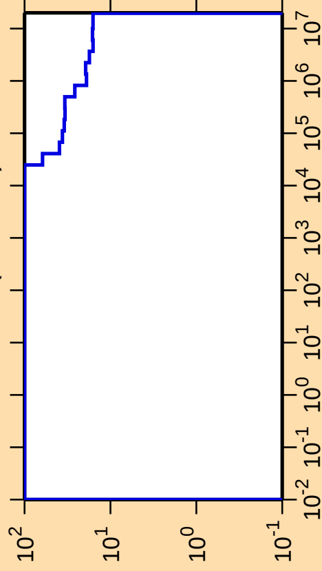
\Delta\sigma/\sigma vs. E for ^{83}\text{Nb}(n,\text{nonel.})
