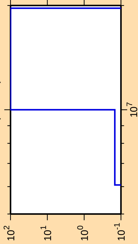
\Delta\sigma/\sigma vs. E for ^{83}\text{Nb}(\text{mt117})
