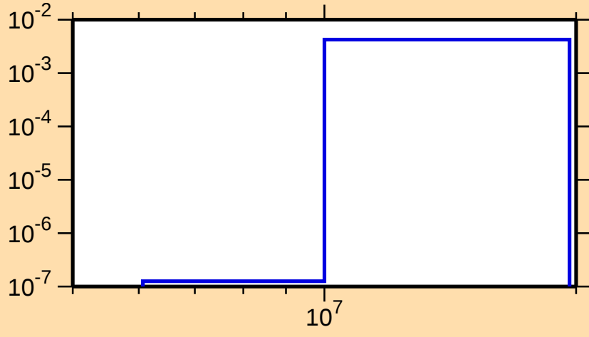
\sigma vs. E for ^{83}\text{Nb}(n,\text{pd})
