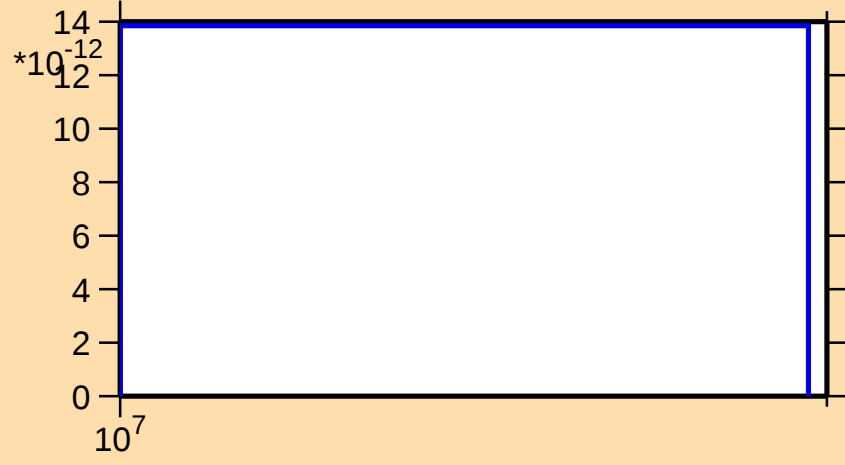
\sigma vs. E for ^{83}\text{Nb}(\text{mt } 34)
