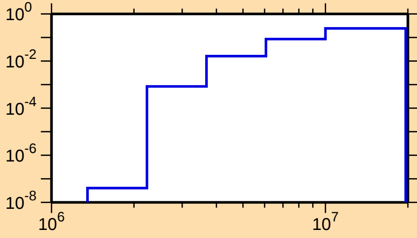
\sigma vs. E for ^{83}\text{Nb}(n,np)
