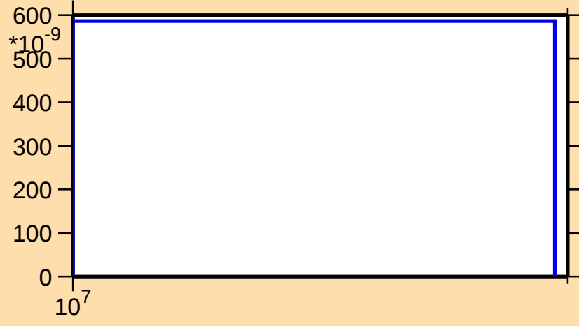
\sigma vs. E for ^{83}\text{Nb}(n,\text{pt})
