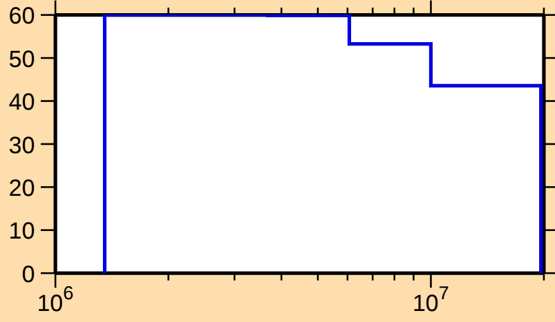
\Delta\sigma/\sigma vs. E for ^{83}\text{Nb}(n,n\text{cont.})
