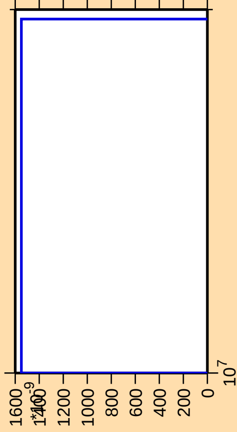
\Delta\sigma/\sigma vs. E for ^{83}\text{Nb}(n,\text{nt})
