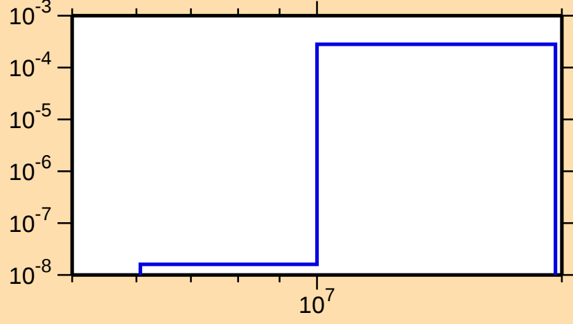
\sigma vs. E for ^{83}\text{Nb}(n,n\alpha)
