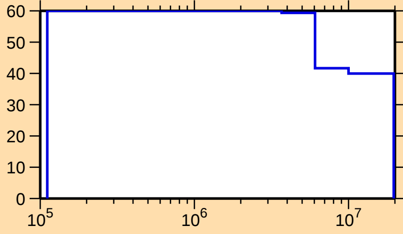
\Delta\sigma/\sigma vs. E for ^{83}\text{Nb}(n,n_1)
