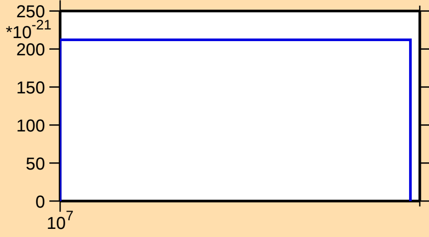
\sigma vs. E for ^{83}\text{Nb}(n,\text{nt})
