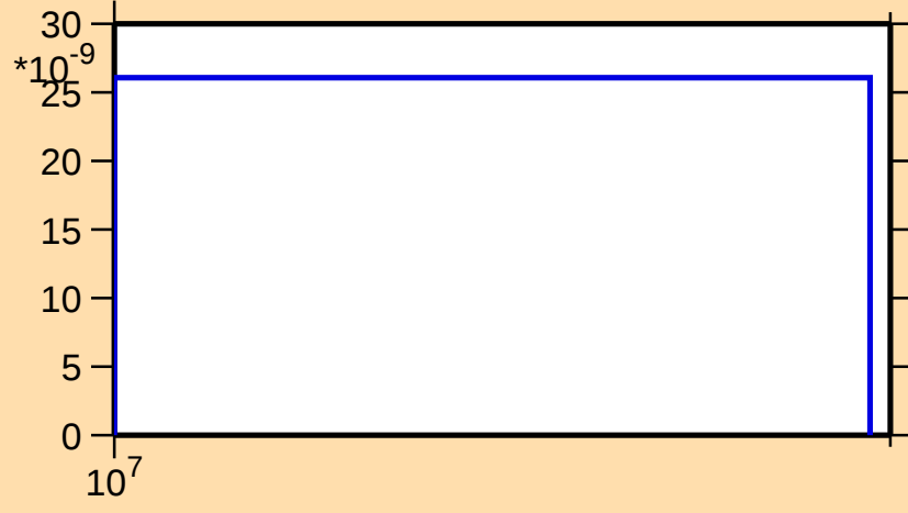
\sigma vs. E for ^{83}\text{Nb}(n,2np)
