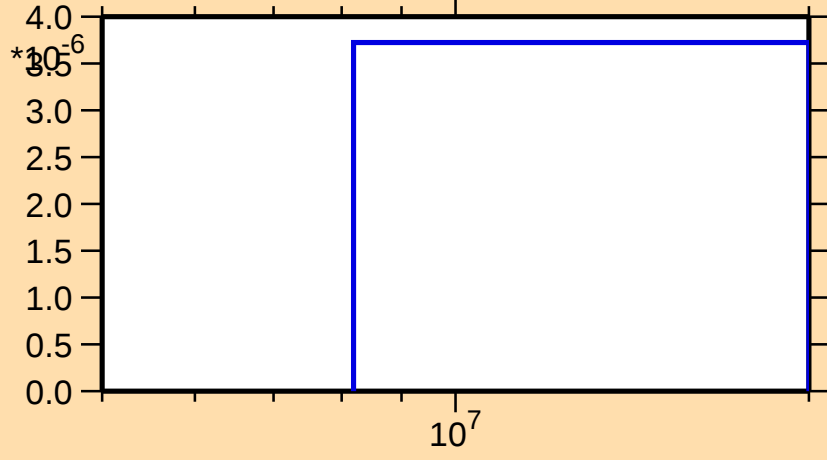
\sigma vs. E for ^{83}\text{Nb}(n,2n)
