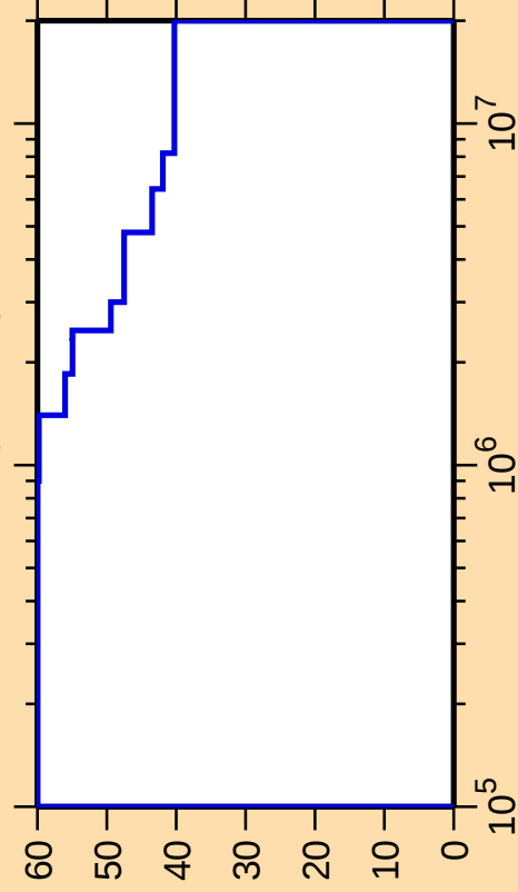
\Delta\sigma/\sigma vs. E for ^{83}\text{Nb}(n,\text{inel.})
