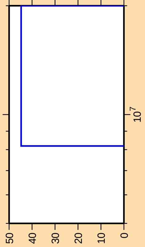
\Delta\sigma/\sigma vs. E for ^{83}\text{Nb}(n,n\text{cont.})
