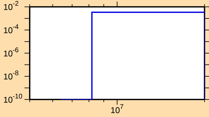
\sigma vs. E for ^{83}\text{Nb}(n,\text{pd})
