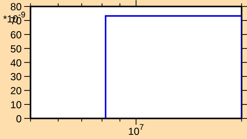
\sigma vs. E for ^{83}\text{Nb}(\text{mt117})
