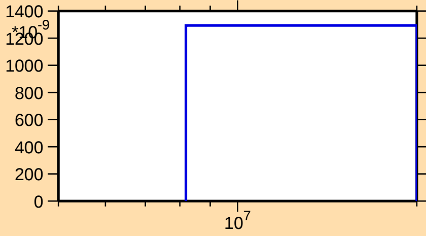
\sigma vs. E for ^{83}\text{Nb}(\text{mt } 45)
