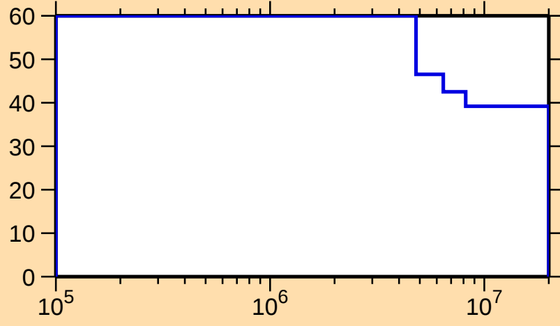
\Delta\sigma/\sigma vs. E for ^{83}\text{Nb}(n,n_1)
