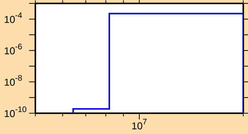
\sigma vs. E for ^{83}\text{Nb}(n,n\alpha)
