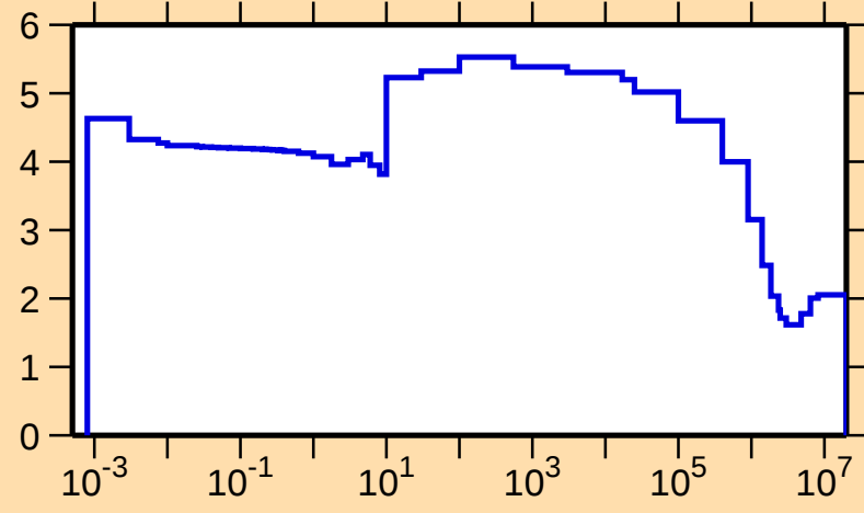
\sigma vs. E for ^{83}\text{Nb}(n,\text{el.})
