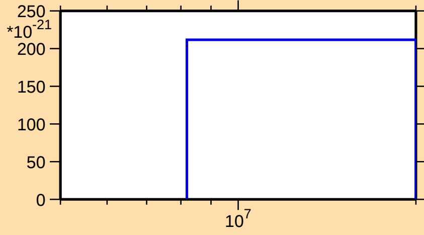
\sigma vs. E for ^{83}\text{Nb}(n,nt)
