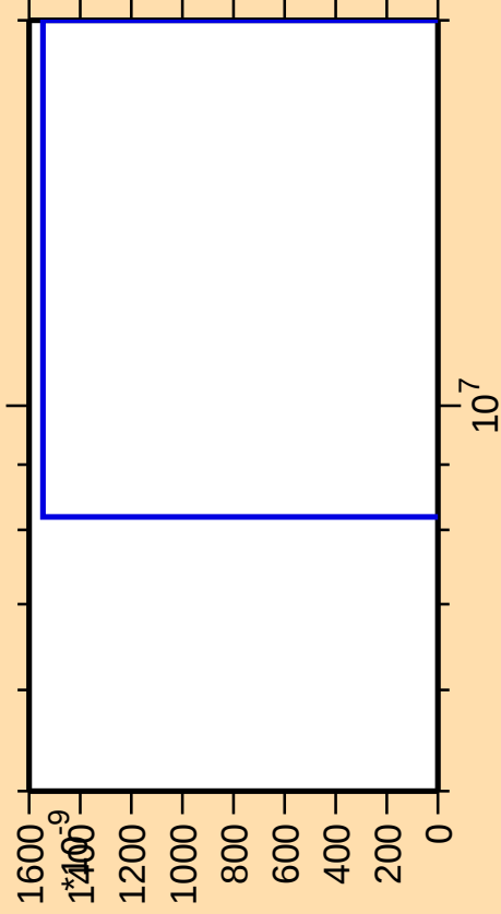
\Delta\sigma/\sigma vs. E for ^{83}\text{Nb}(n,nt)
