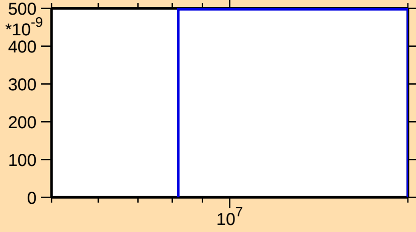
\sigma vs. E for ^{83}\text{Nb}(n,\text{pt})
