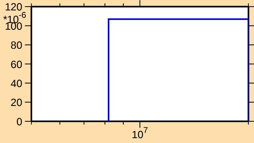
\sigma vs. E for ^{83}\text{Nb}(n,t)
