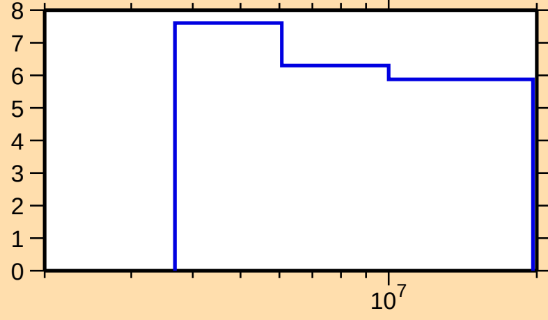
\Delta\sigma/\sigma vs. E for ^{88}\text{Nb}(n,n\text{nonel.})
