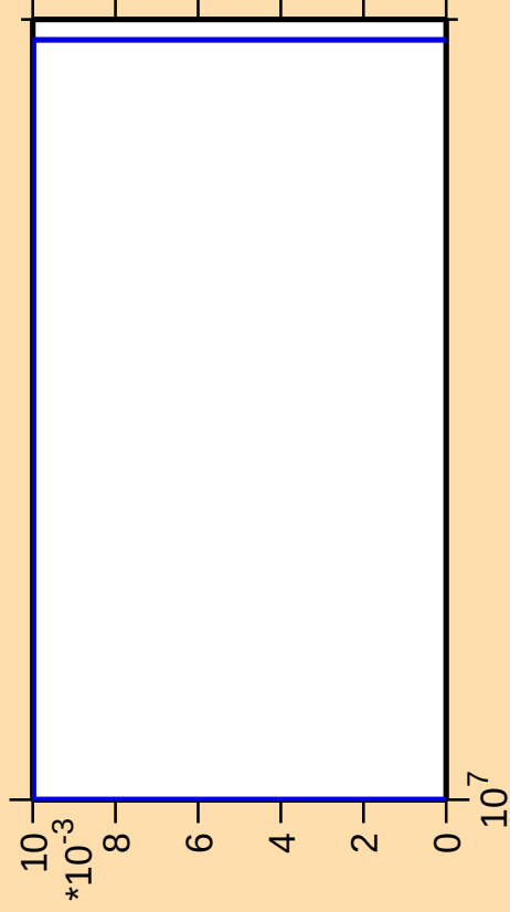
\Delta\sigma/\sigma vs. E for ^{89}\text{Nb}(n,\text{nt})
