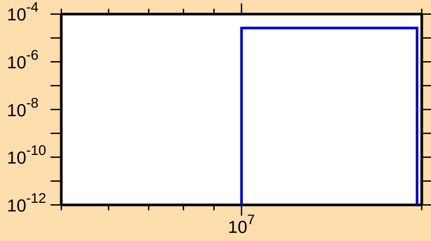
\sigma vs. E for ^{89}\text{Nb}(n,t)
