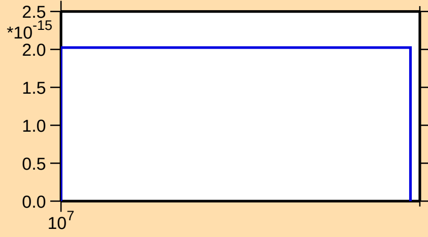
\sigma vs. E for ^{89}\text{Nb}(n,\text{nt})
