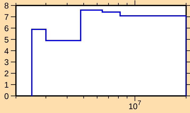
\Delta\sigma/\sigma vs. E for ^{89}\text{Nb}(n,n\text{onel.})
