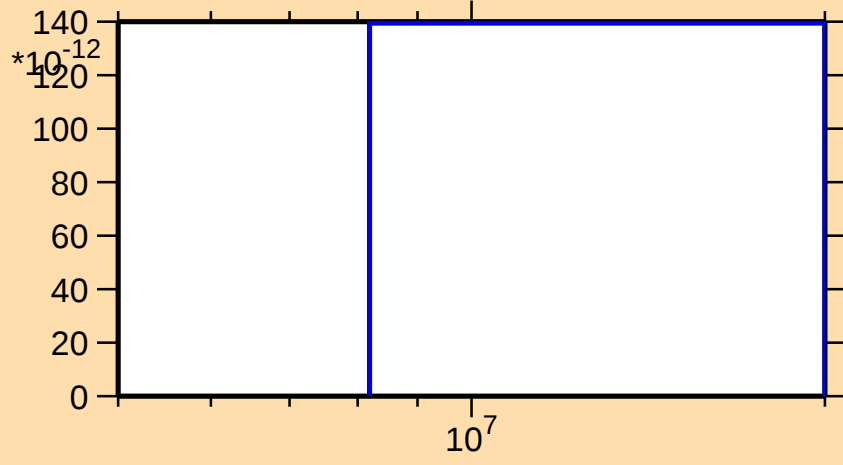
\sigma vs. E for ^{89}\text{Nb}(\text{mt } 45)
