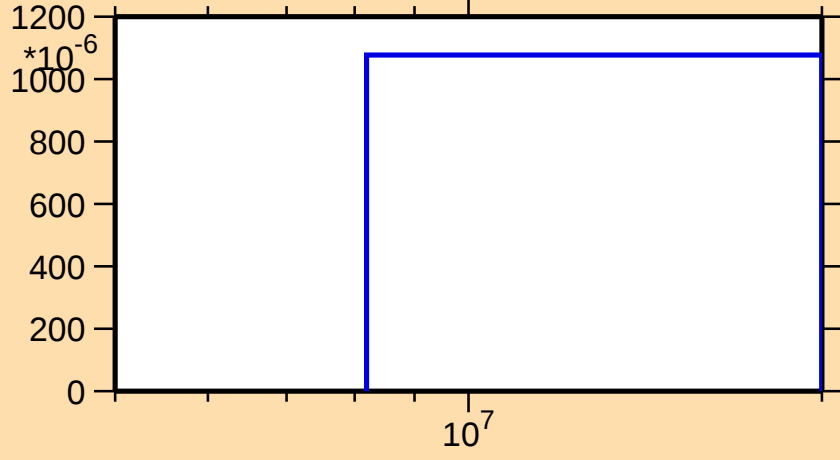
\sigma vs. E for ^{89}\text{Nb}(n,n\alpha)
