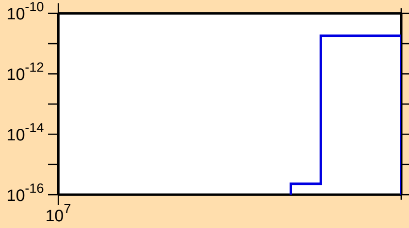
\sigma vs. E for ^{90}\text{Nb}(\text{mt } 45)
