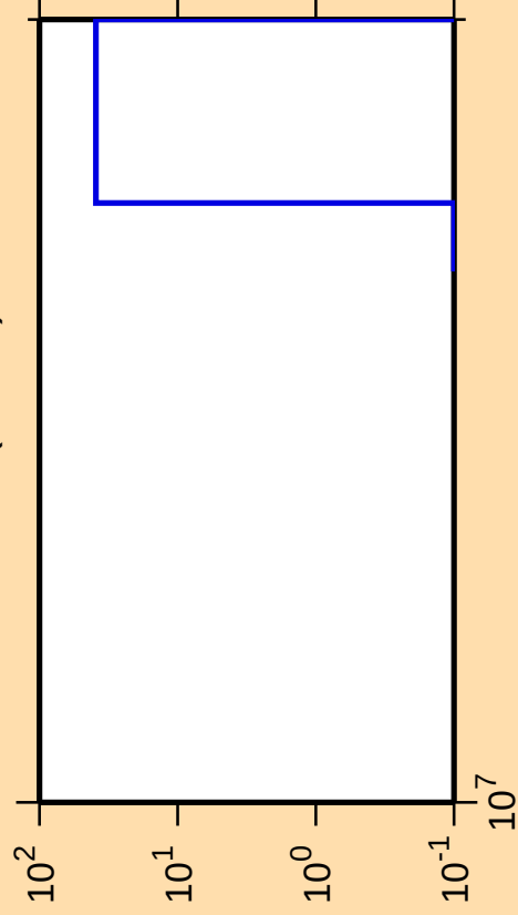
\Delta\sigma/\sigma vs. E for ^{90}\text{Nb}(\text{mt } 45)
