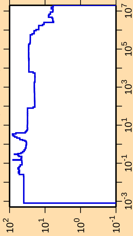
\Delta\sigma/\sigma vs. E for ^{90}\text{Nb}(n,\text{nonel.})
