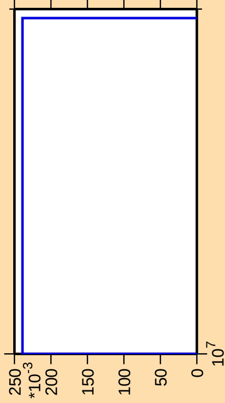
\Delta\sigma/\sigma vs. E for ^{90}\text{Nb}(\text{mt } 45)
