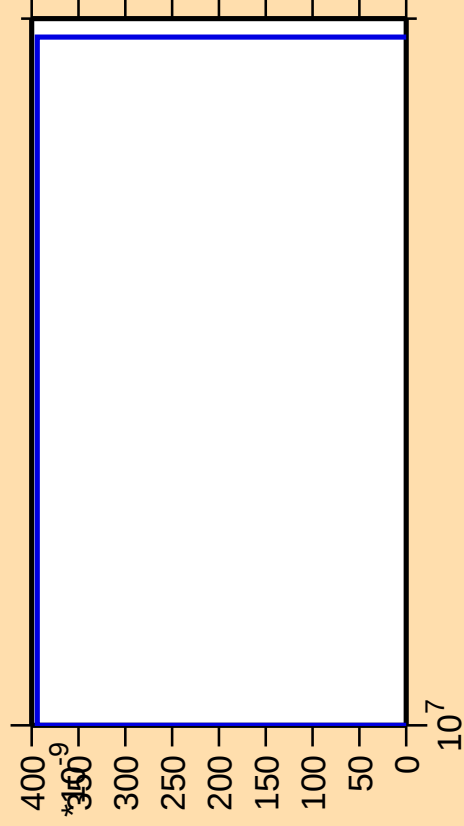
\Delta\sigma/\sigma vs. E for ^{90}\text{Nb}(n,nt)
