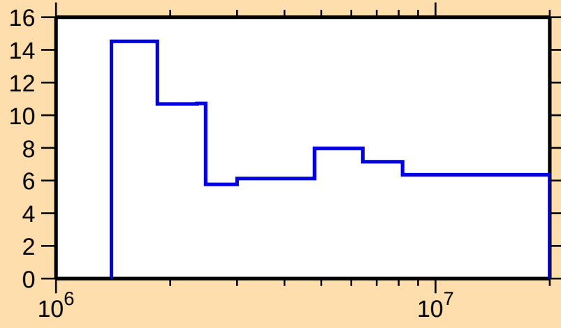
\Delta\sigma/\sigma vs. E for ^{90}\text{Nb}(n,n\text{nonel.})
