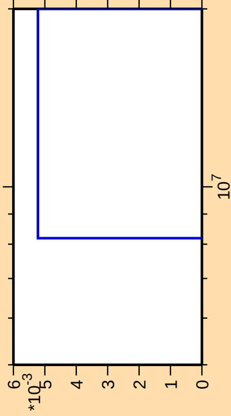
\Delta\sigma/\sigma vs. E for ^{90}\text{Nb}(\text{mt } 34)
