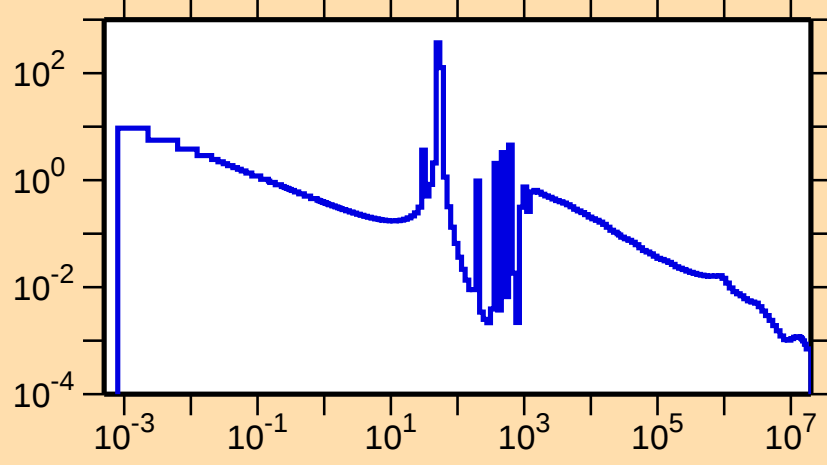
\sigma vs. E for ^{91}\text{Nb}(n,\gamma)
