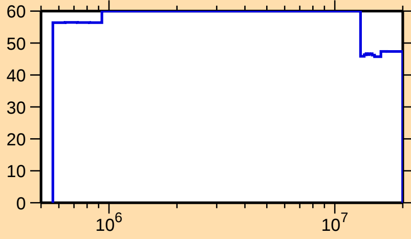
\Delta\sigma/\sigma vs. E for ^{91}\text{Nb}(n,p)
