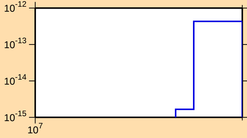
\sigma vs. E for ^{91}\text{Nb}(\text{mt117})
