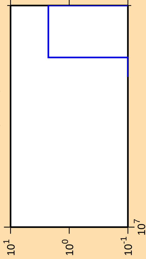
\Delta\sigma/\sigma vs. E for ^{91}\text{Nb}(\text{mt } 45)
