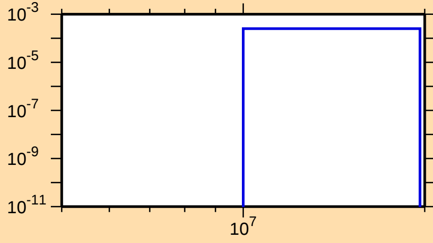
\sigma vs. E for ^{91}\text{Nb}(n,n\alpha)
