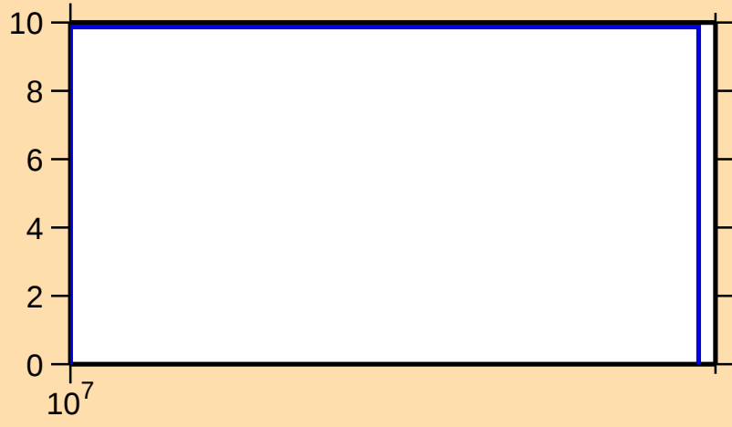
\Delta\sigma/\sigma vs. E for ^{91}\text{Nb}(n,\text{el.})
