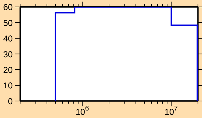
\Delta\sigma/\sigma vs. E for ^{91}\text{Nb}(n,p)
