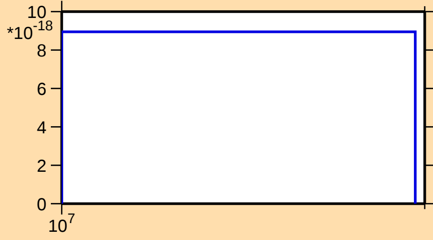
\sigma vs. E for ^{91}\text{Nb}(n,\text{nt})
