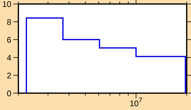
\Delta\sigma/\sigma vs. E for ^{91}\text{Nb}(n,n\text{nonel.})
