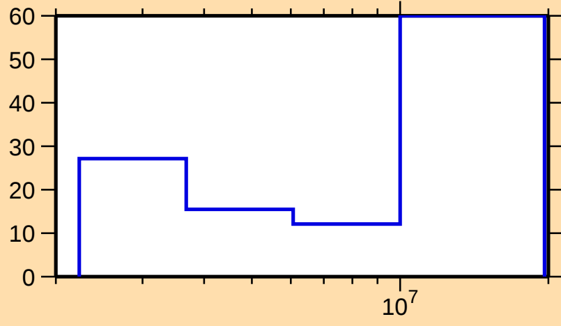
\Delta\sigma/\sigma vs. E for ^{91}\text{Nb}(n,n\text{cont.})
