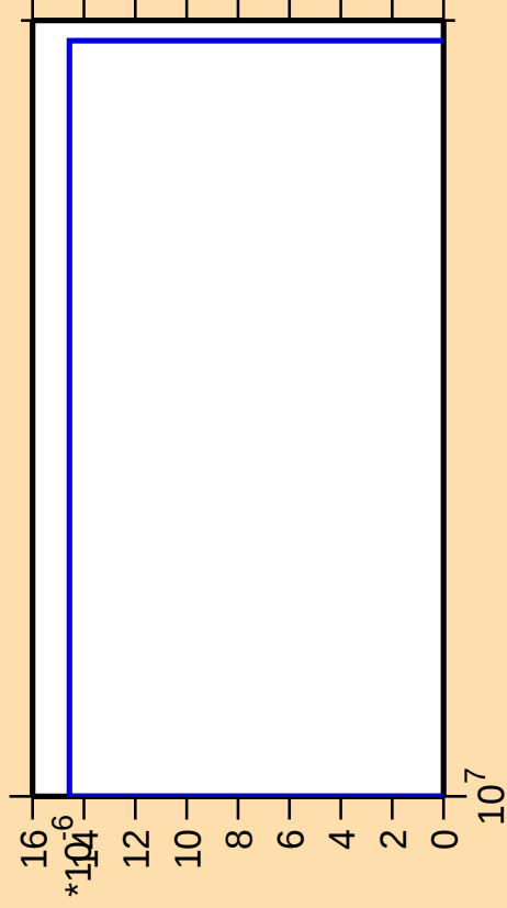
\Delta\sigma/\sigma vs. E for ^{91}\text{Nb}(n,\text{nt})
