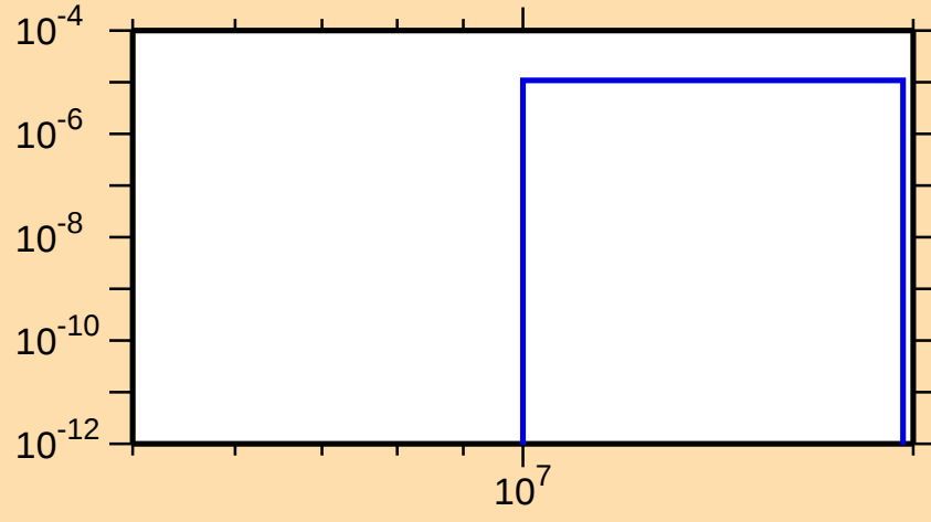
\sigma vs. E for ^{91}\text{Nb}(n,t)
