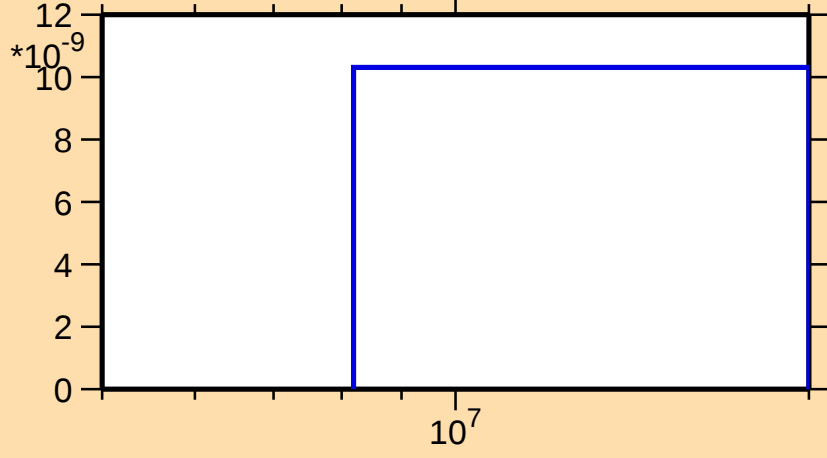
\sigma vs. E for ^{91}\text{Nb}(n,\text{nd})
