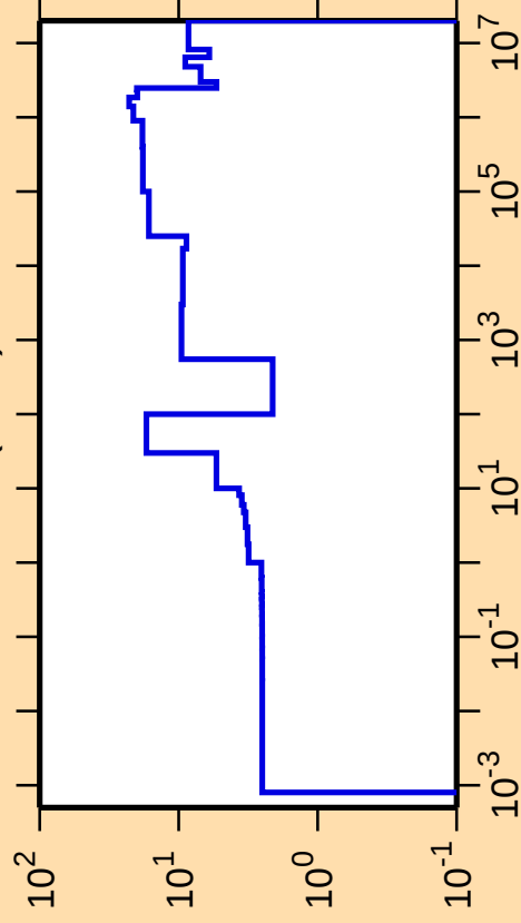
\Delta\sigma/\sigma vs. E for ^{91}\text{Nb}(n,\text{el.})
