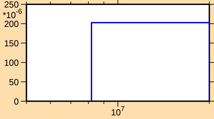
\sigma vs. E for ^{91}\text{Nb}(n,n\alpha)
