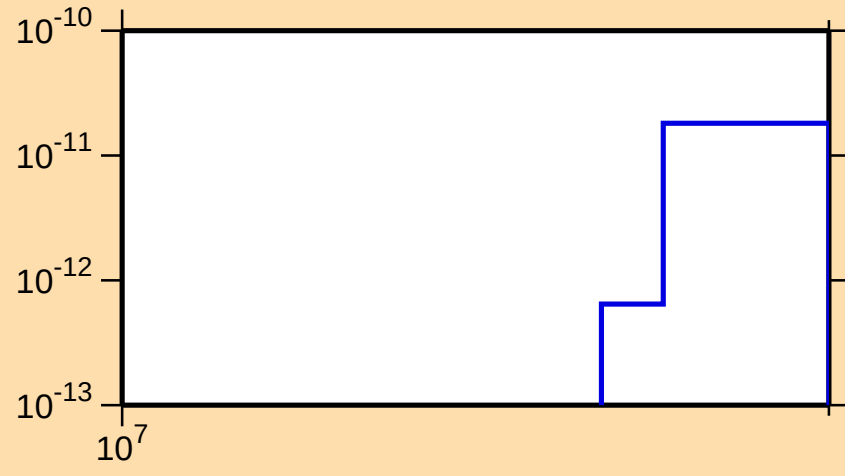
\sigma vs. E for ^{94}\text{Nb}(\text{mt117})
