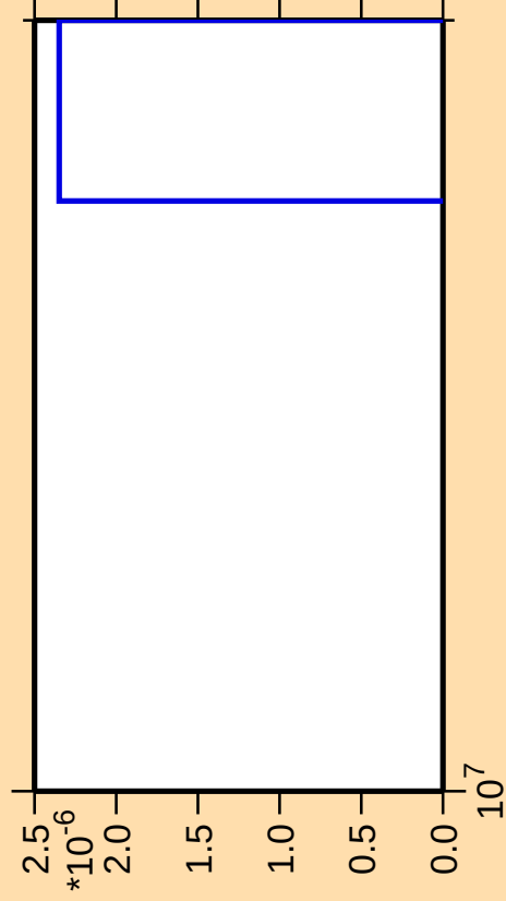
\Delta\sigma/\sigma vs. E for ^{94}\text{Nb}(\text{mt } 11)
