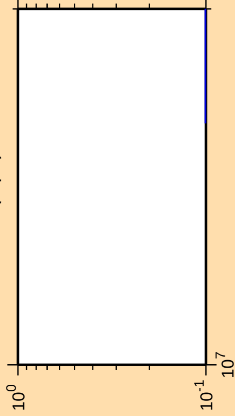
\Delta\sigma/\sigma vs. E for ^{94}\text{Nb}(n,\text{pd})
