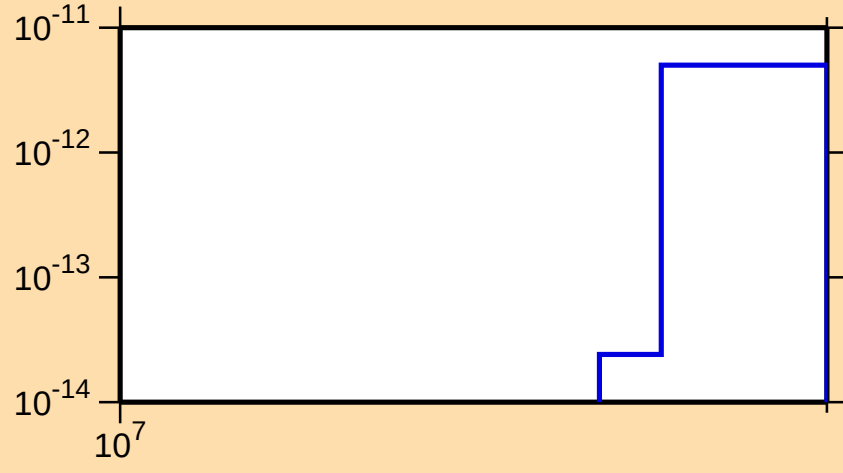
\sigma vs. E for ^{94}\text{Nb}(\text{mt } 45)
