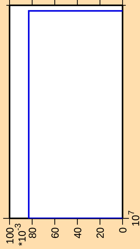
\Delta\sigma/\sigma vs. E for ^{94}\text{Nb}(\text{mt } 45)
