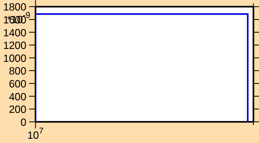
\sigma vs. E for ^{94}\text{Nb}(n,2n\alpha)
