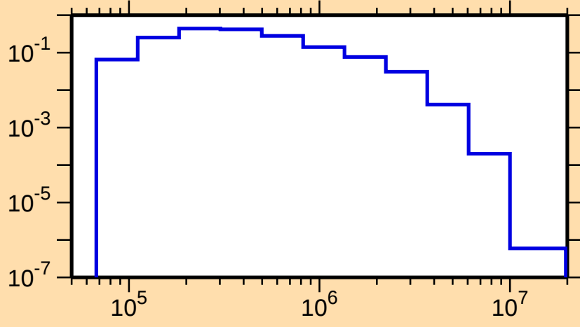
\sigma vs. E for ^{94}\text{Nb}(n,n_4)
