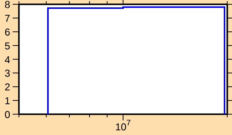
\Delta\sigma/\sigma vs. E for ^{94}\text{Nb}(n,\text{el.})
