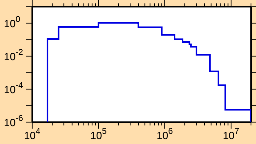
\sigma vs. E for ^{94}\text{Nb}(n,n_2)
