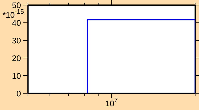
\sigma vs. E for ^{94}\text{Nb}(\text{mt } 45)
