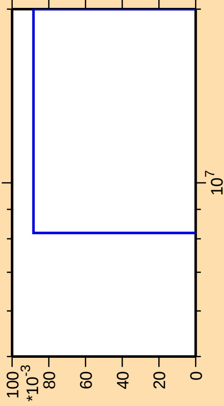
\Delta\sigma/\sigma vs. E for ^{94}\text{Nb}(\text{mt } 45)
