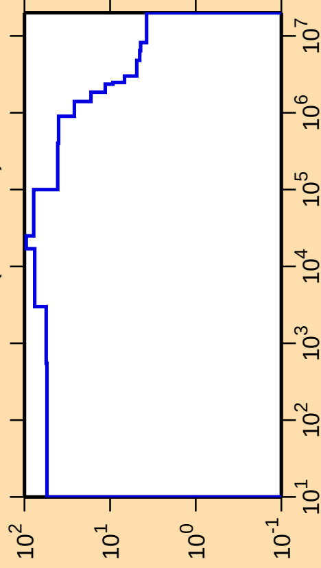
\Delta\sigma/\sigma vs. E for ^{95}\text{Nb}(n,\text{nonel.})
