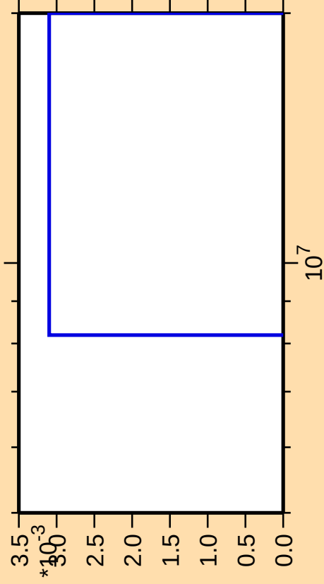
\Delta\sigma/\sigma vs. E for ^{95}\text{Nb}(\text{mt } 45)
