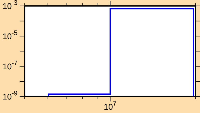
\sigma vs. E for ^{96}\text{Nb}(n,n\alpha)
