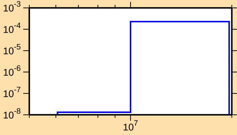
\sigma vs. E for ^{96}\text{Nb}(n,t)
