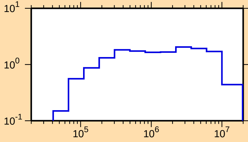
\sigma vs. E for ^{96}\text{Nb}(n,\text{inel.})
