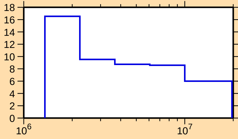
\Delta\sigma/\sigma vs. E for ^{96}\text{Nb}(n,n\text{nonel.})
