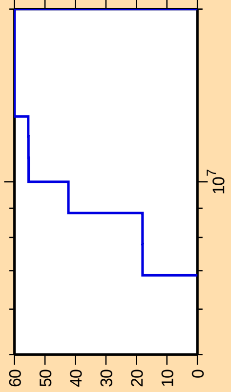
\Delta\sigma/\sigma vs. E for ^{97}\text{Nb}(n,n\text{cont.})
