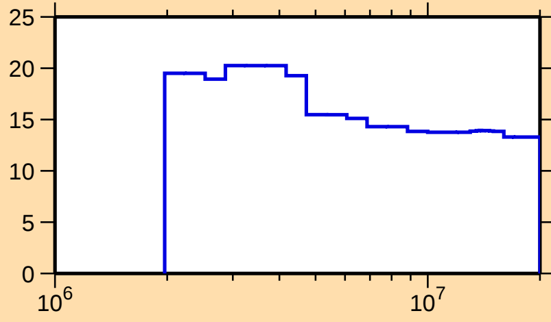
\Delta\sigma/\sigma vs. E for ^{97}\text{Nb}(n,n\text{oncl.})
