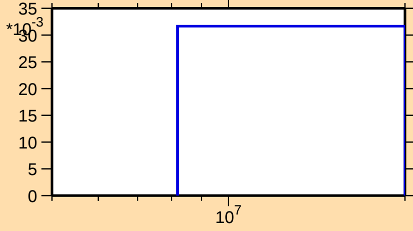
\sigma vs. E for ^{97}\text{Nb}(n,3n)
