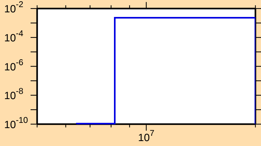
\sigma vs. E for ^{97}\text{Nb}(n,np)
