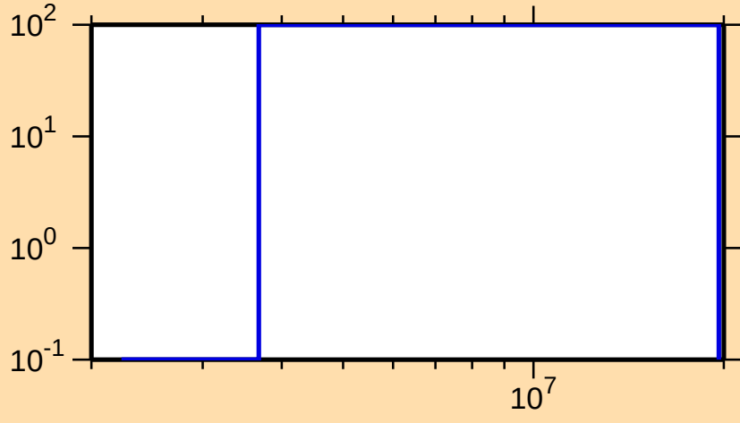
\Delta\sigma/\sigma vs. E for ^{100}\text{Nb}(n,p)
