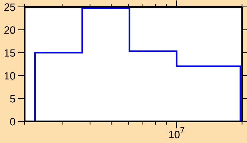
\Delta\sigma/\sigma vs. E for ^{100}\text{Nb}(n,\text{el.})
