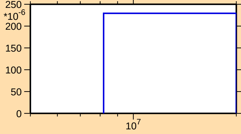
\sigma vs. E for ^{100}\text{Nb}(n,np)
