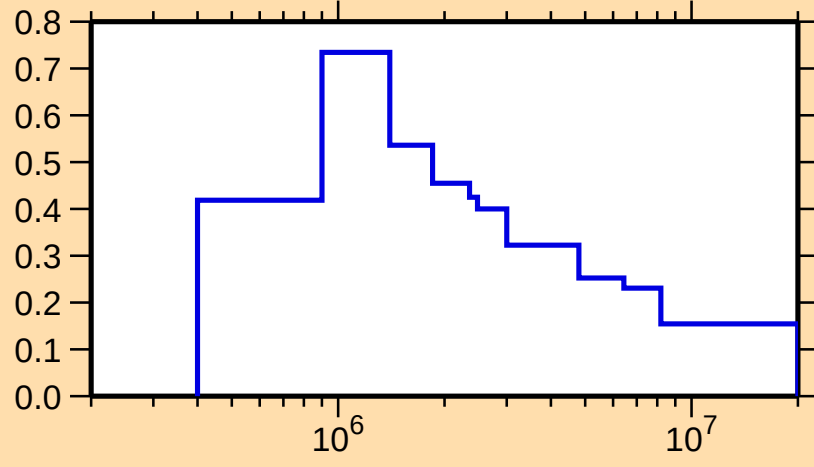
\sigma vs. E for ^{100}\text{Nb}(n,n_4)
