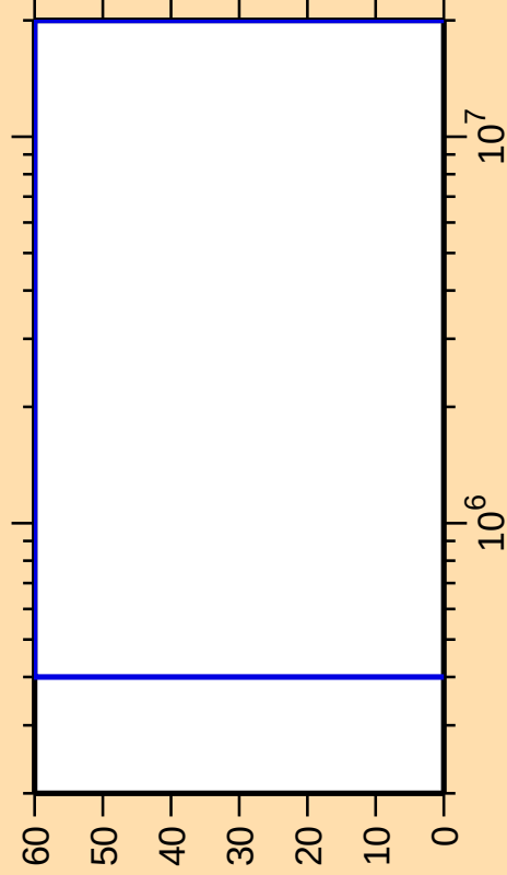
\Delta\sigma/\sigma vs. E for ^{100}\text{Nb}(n,n_4)
