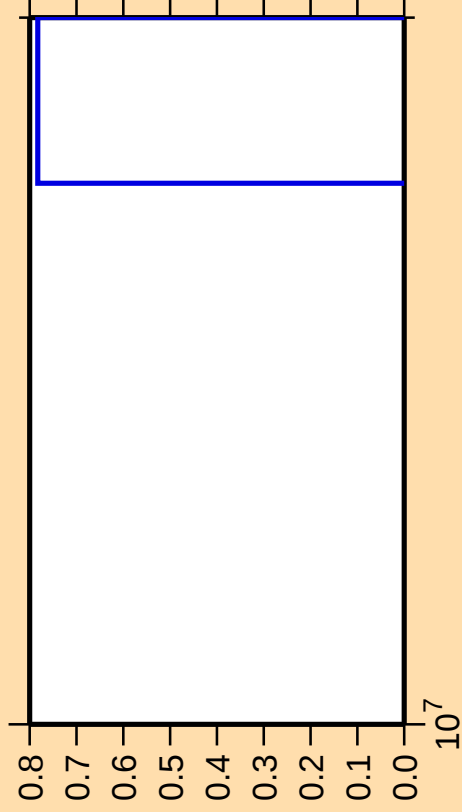
\Delta\sigma/\sigma vs. E for ^{100}\text{Nb}(\text{mt } 11)
