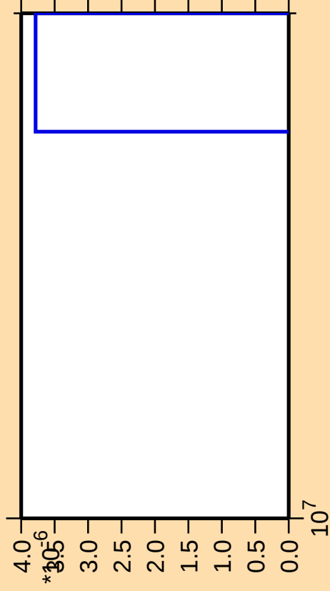
\Delta\sigma/\sigma vs. E for ^{100}\text{Nb}(\text{mt } 34)
