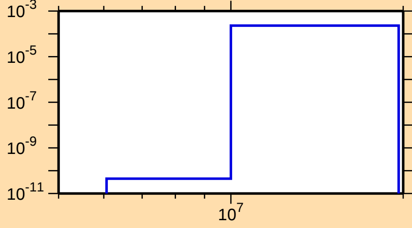
\sigma vs. E for ^{100}\text{Nb}(n,t)
