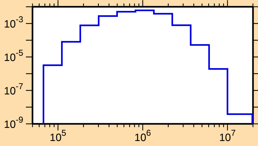
\sigma vs. E for ^{100}\text{Nb}(n,n_2)
