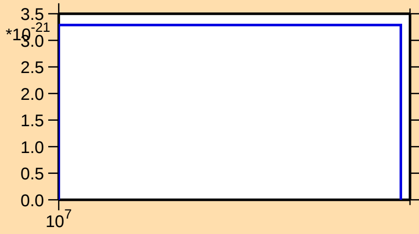
\sigma vs. E for ^{100}\text{Nb}(\text{mt } 34)
