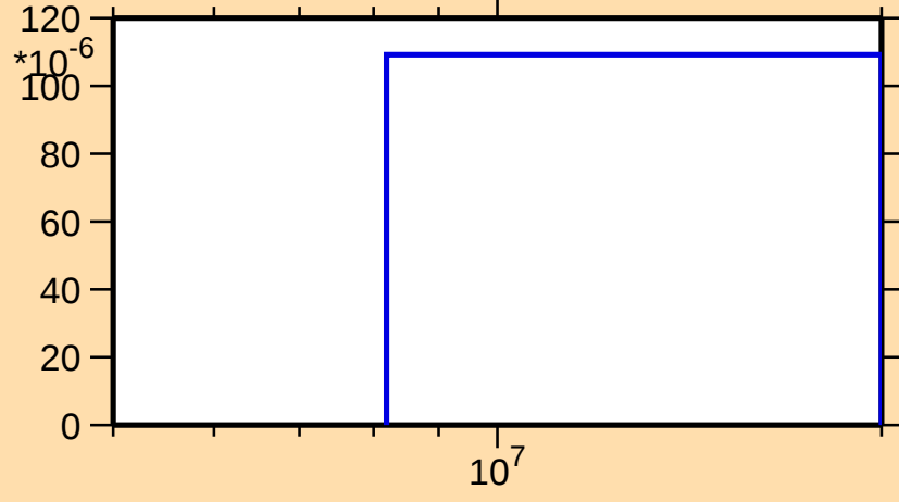
\sigma vs. E for ^{101}\text{Nb}(n,np)
