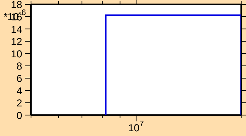
\sigma vs. E for ^{101}\text{Nb}(n,t)
