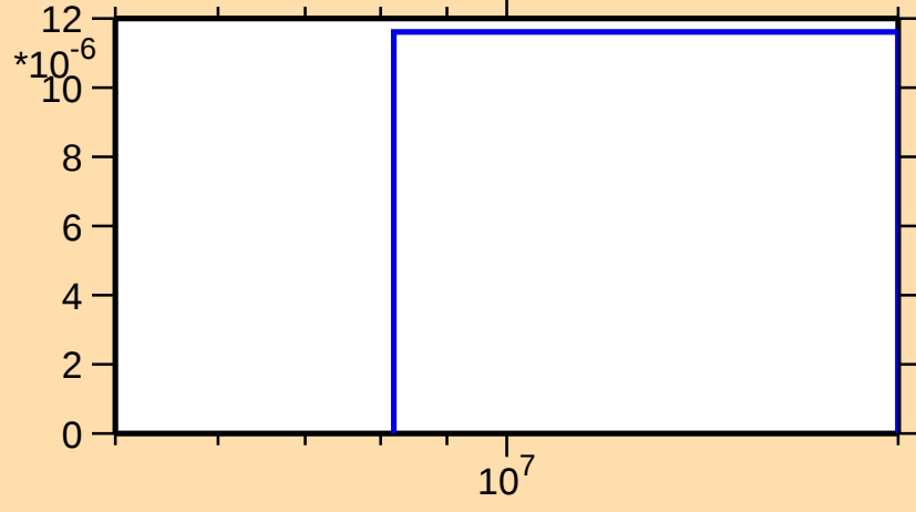
\sigma vs. E for ^{101}\text{Nb}(n,n\alpha)
