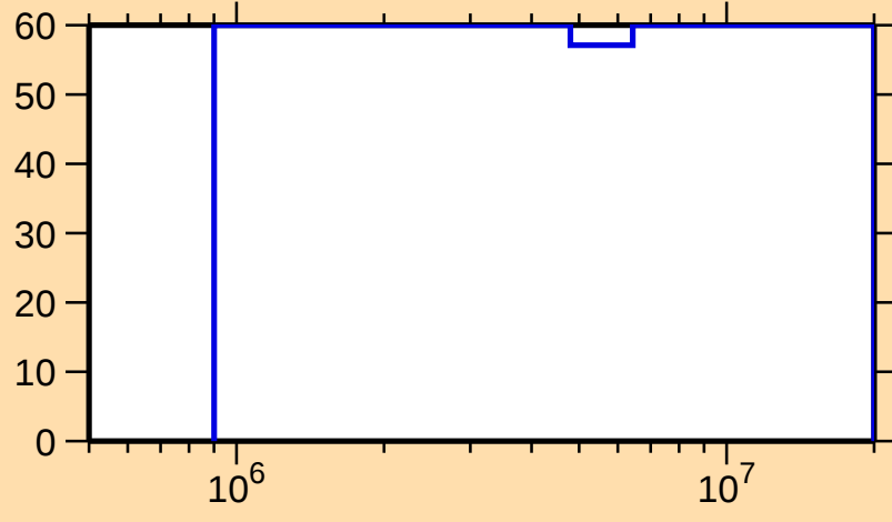
\Delta\sigma/\sigma vs. E for ^{101}\text{Nb}(n,n_1)
