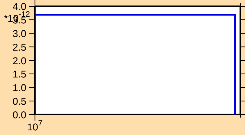
\sigma vs. E for ^{130}\text{Nd}(\text{mt } 34)
