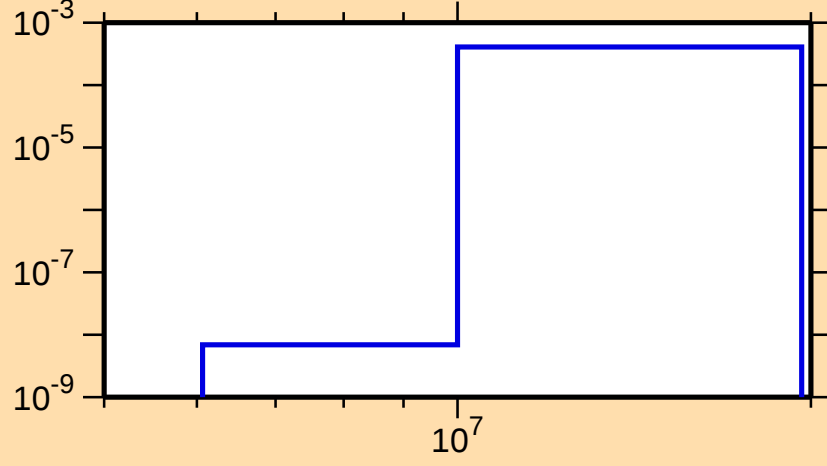
\sigma vs. E for ^{130}\text{Nd}(n,\text{pd})
