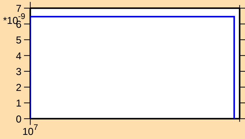
\sigma vs. E for ^{130}\text{Nd}(n,\text{pt})
