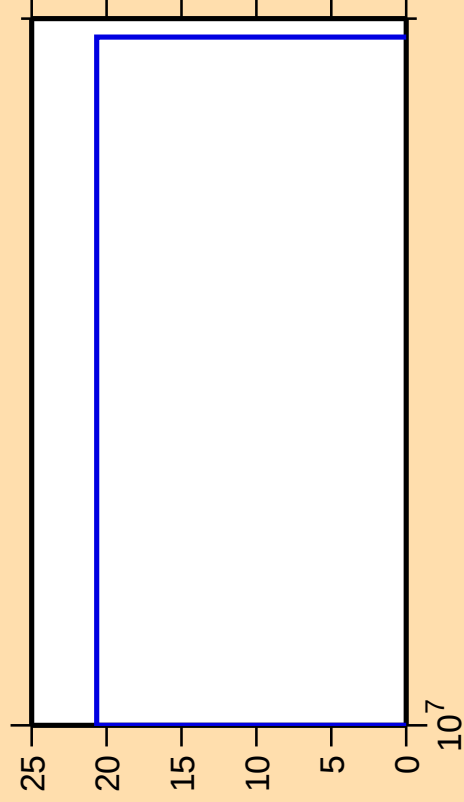
\Delta\sigma/\sigma vs. E for ^{130}\text{Nd}(\text{mt } 34)
