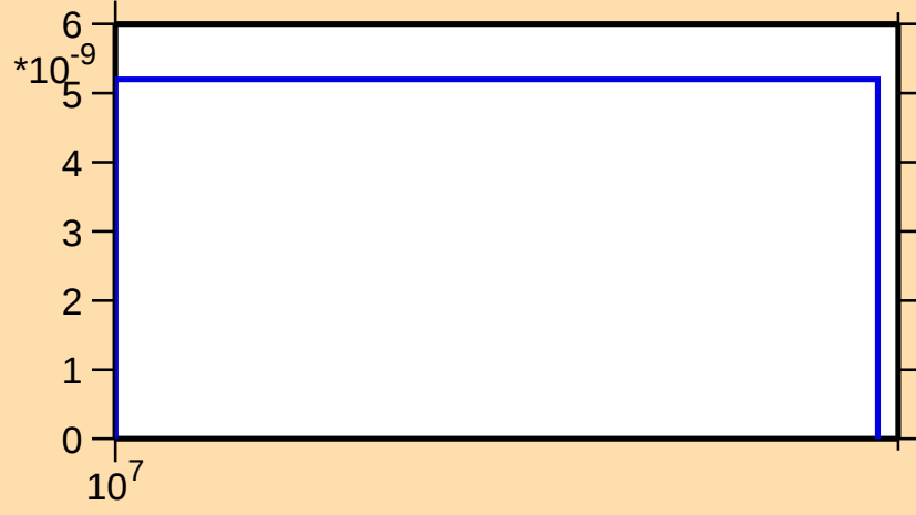
\sigma vs. E for ^{130}\text{Nd}(n,2np)
