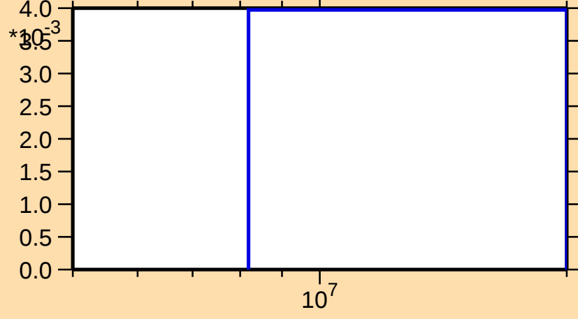
\sigma vs. E for ^{130}\text{Nd}(n,2n)
