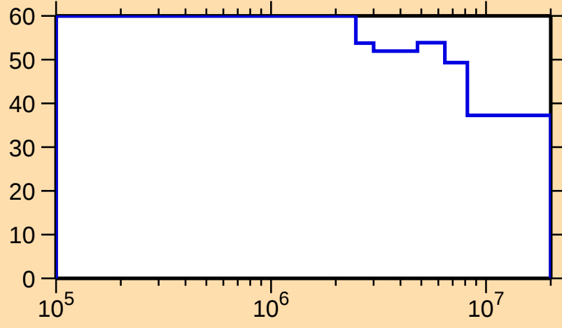
\Delta\sigma/\sigma vs. E for ^{130}\text{Nd}(n,n_1)
