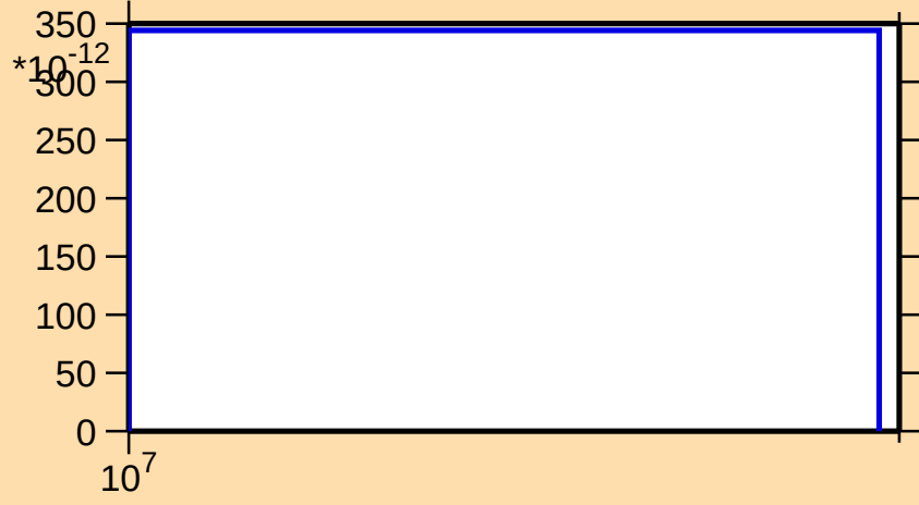
\sigma vs. E for ^{133}\text{Nd} (mt 34)
