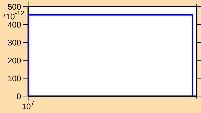
\sigma vs. E for ^{133}\text{Nd}(\text{mt117})
