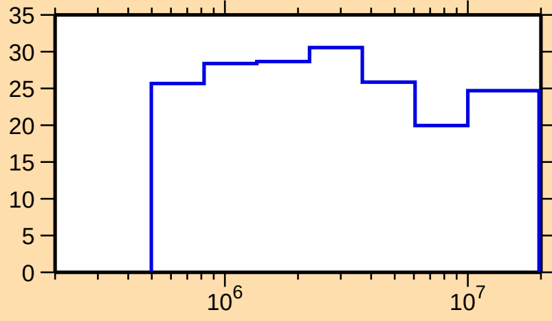
\Delta\sigma/\sigma vs. E for ^{133}\text{Nd}(n,n\text{nonel.})
