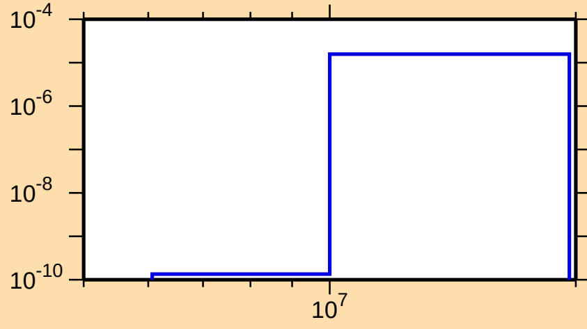
\sigma vs. E for ^{133}\text{Nd}(n,\text{He3})
