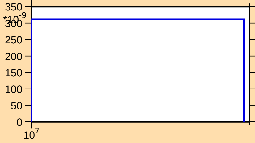
\sigma vs. E for ^{133}\text{Nd}(n,\text{pt})
