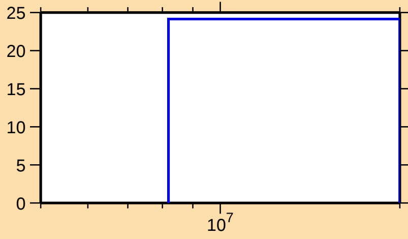
\Delta\sigma/\sigma vs. E for ^{133}\text{Nd}(n,\text{nonel.})
