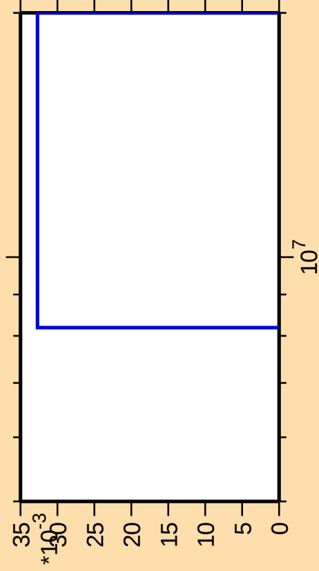
\Delta\sigma/\sigma vs. E for ^{133}\text{Nd}(n,\text{nt})
