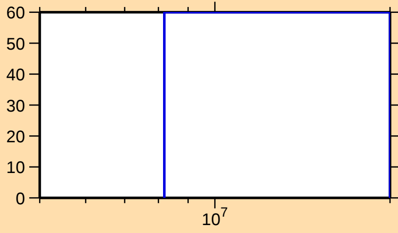
\Delta\sigma/\sigma vs. E for ^{133}\text{Nd}(n,2n)
