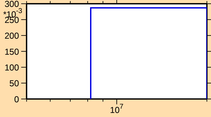
\sigma vs. E for ^{133}\text{Nd}(n,2n)
