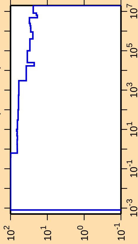
\Delta\sigma/\sigma vs. E for ^{133}\text{Nd}(n,\text{nonel.})
