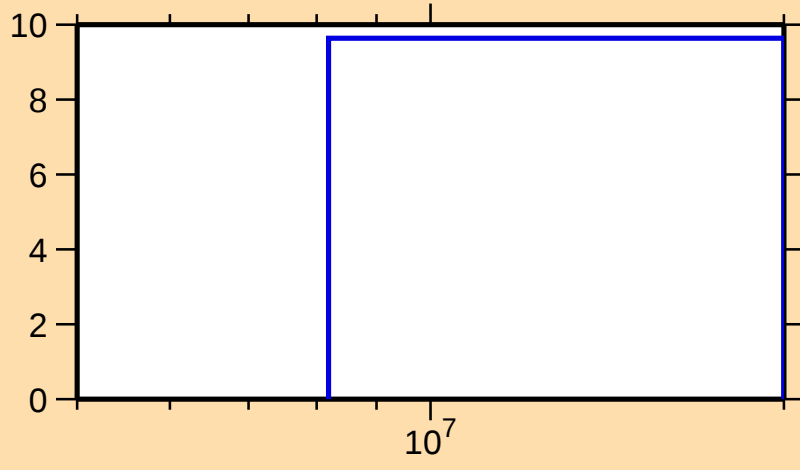
\Delta\sigma/\sigma vs. E for ^{133}\text{Nd}(n,\text{el.})
