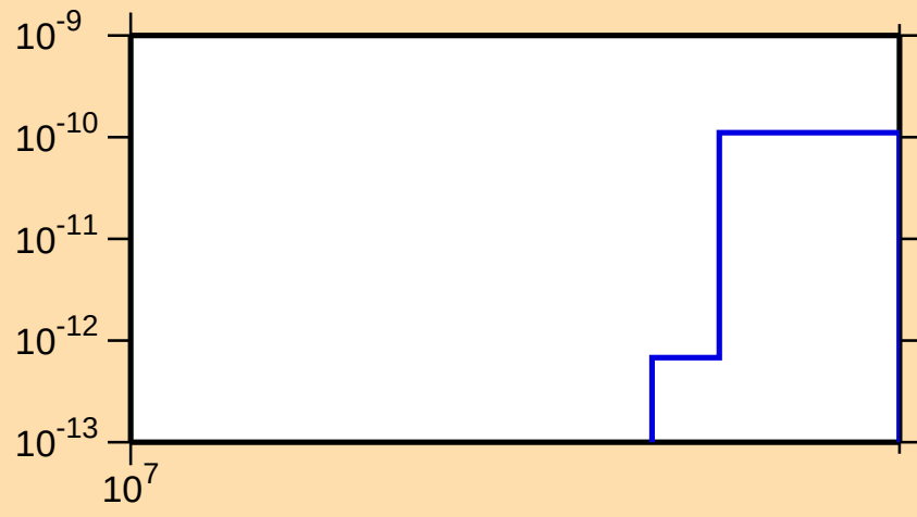
\sigma vs. E for ^{137}\text{Nd} (mt 34)
