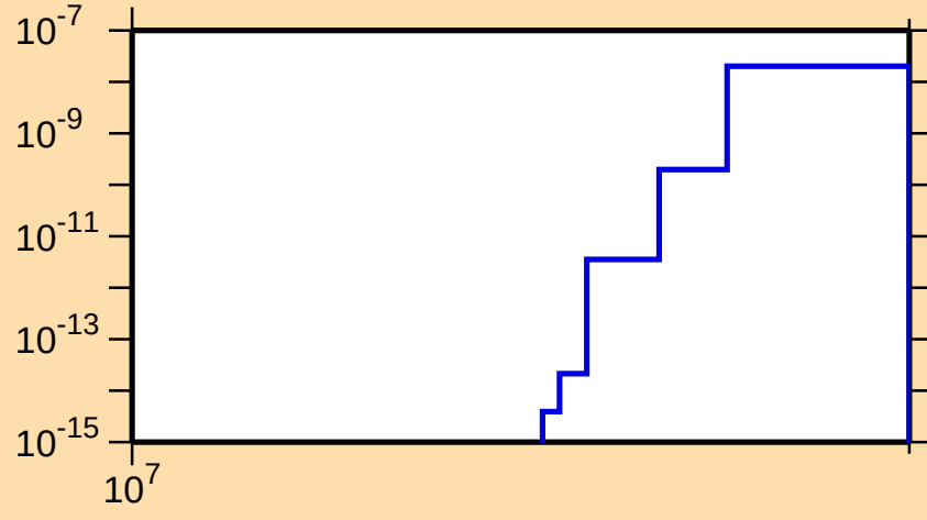
\sigma vs. E for ^{137}\text{Nd}(n,\text{pt})
