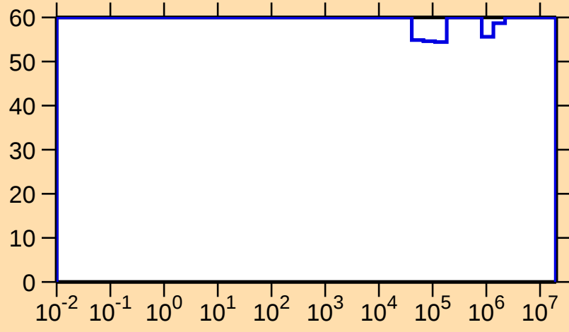
\Delta\sigma/\sigma vs. E for ^{137}\text{Nd}(n,p)
