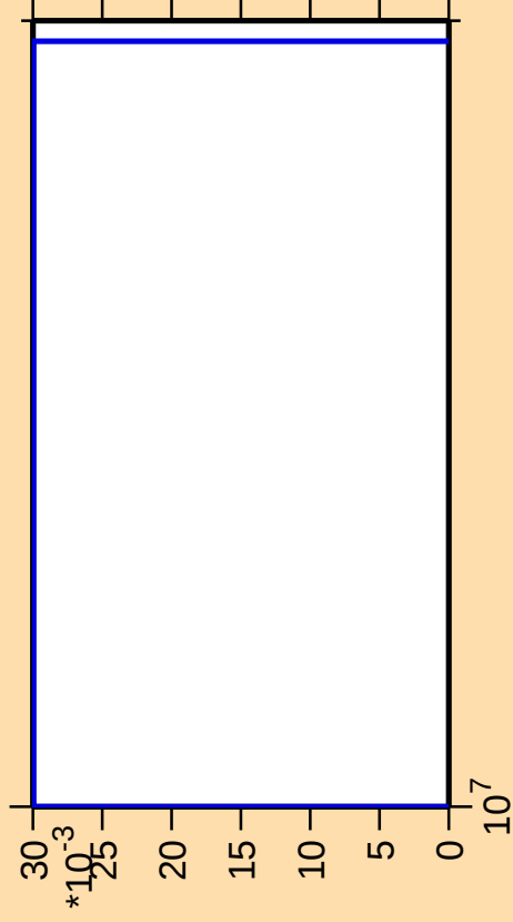
\Delta\sigma/\sigma vs. E for ^{137}\text{Nd}(n,\text{nt})
