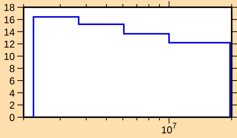
\Delta\sigma/\sigma vs. E for ^{137}\text{Nd}(n,n\text{onel.})
