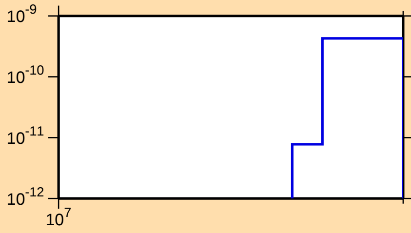
\sigma vs. E for ^{137}\text{Nd}(\text{mt } 45)
