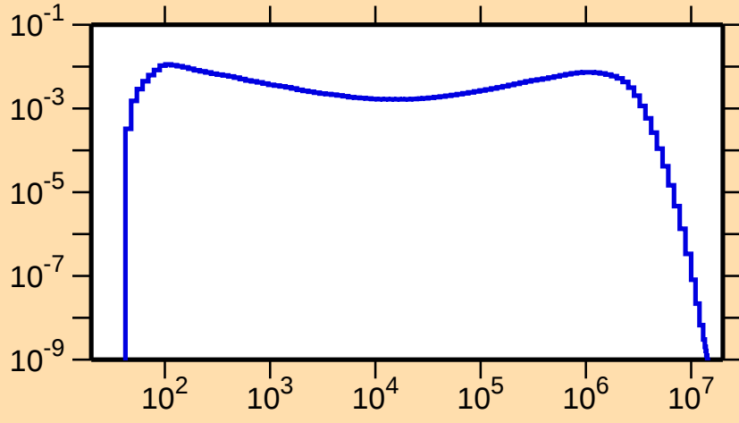
\sigma vs. E for ^{137}\text{Nd}(n,n_2)
