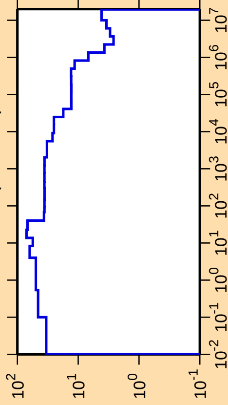
\Delta\sigma/\sigma vs. E for ^{137}\text{Nd}(n,\text{nonel.})
