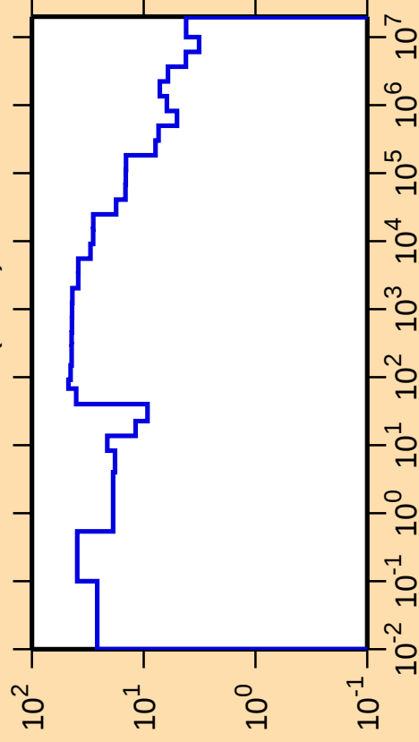
\Delta\sigma/\sigma vs. E for ^{137}\text{Nd}(n,\text{el.})
