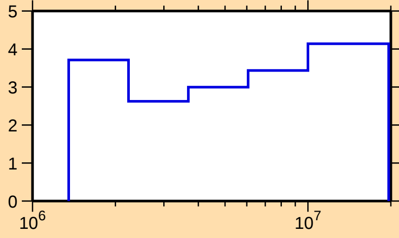
\Delta\sigma/\sigma vs. E for ^{137}\text{Nd}(n,n\text{nonel.})
