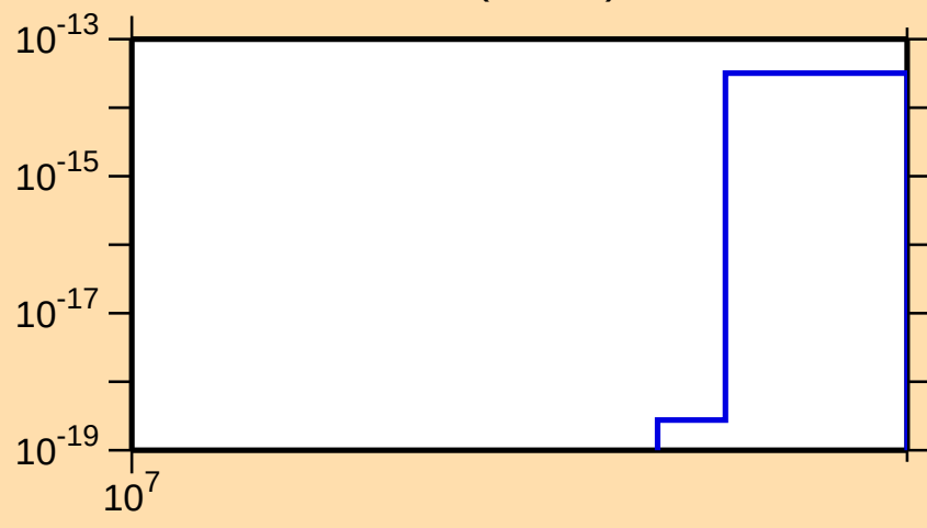
\sigma vs. E for ^{138}\text{Nd} (mt 34)
