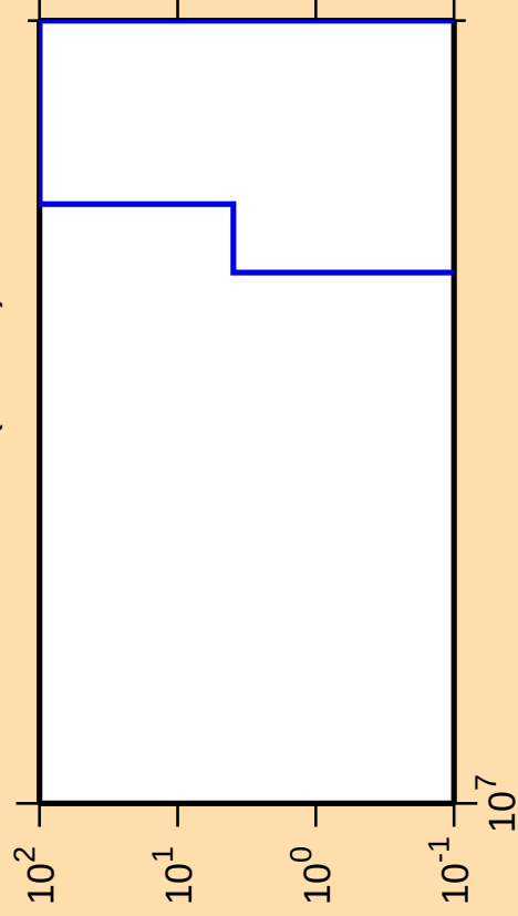
\Delta\sigma/\sigma vs. E for ^{138}\text{Nd} (mt 45)
