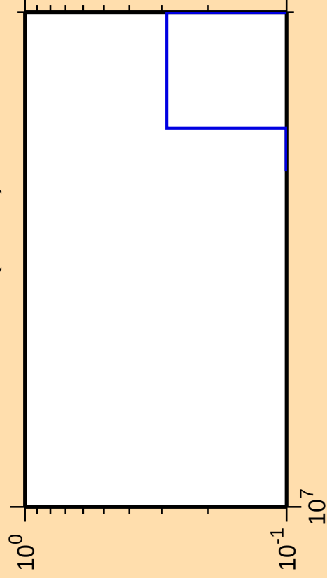
\Delta\sigma/\sigma vs. E for ^{138}\text{Nd} (mt 34)
