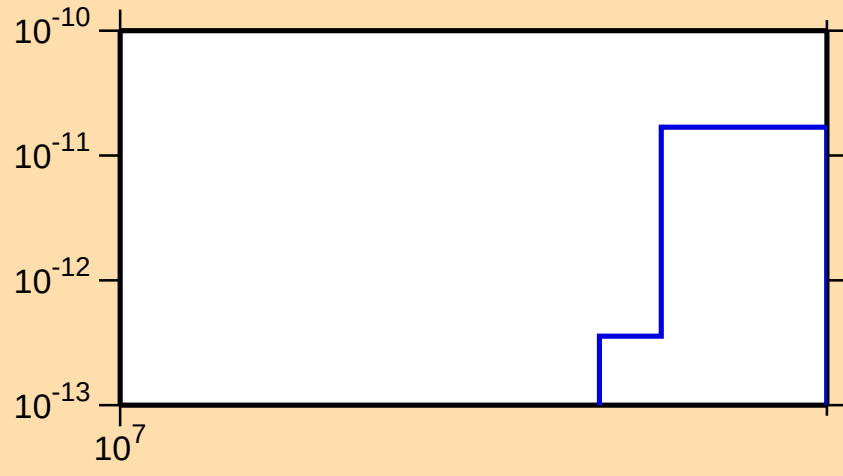
\sigma vs. E for ^{138}\text{Nd}(\text{mt117})
