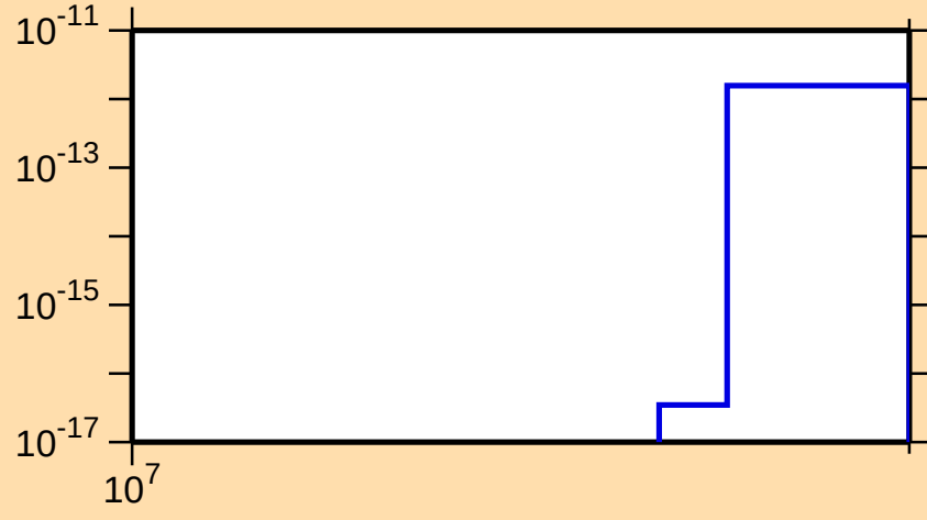
\sigma vs. E for ^{138}\text{Nd}(n,\text{pt})
