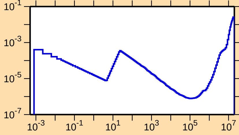
\sigma vs. E for ^{138}\text{Nd}(n,\alpha)
