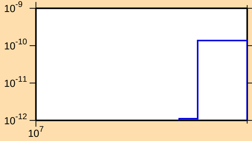
\sigma vs. E for ^{138}\text{Nd} (mt 45)
