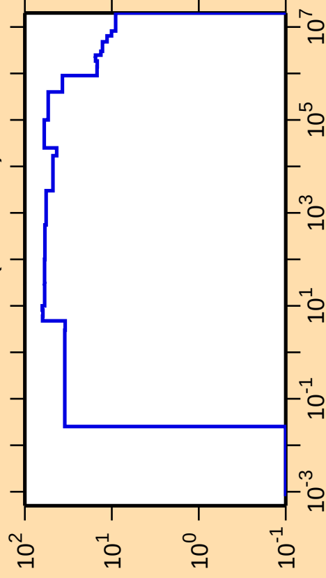
\Delta\sigma/\sigma vs. E for ^{138}\text{Nd}(n,\text{nonel.})
