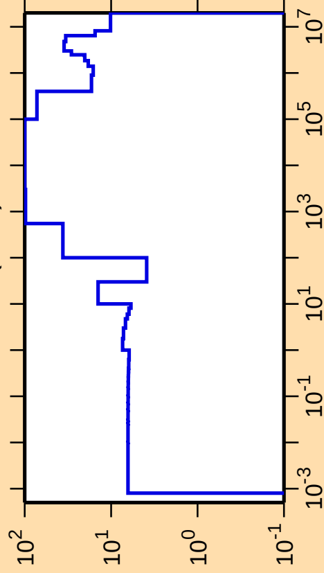
\Delta\sigma/\sigma vs. E for ^{138}\text{Nd}(n,\text{el.})
