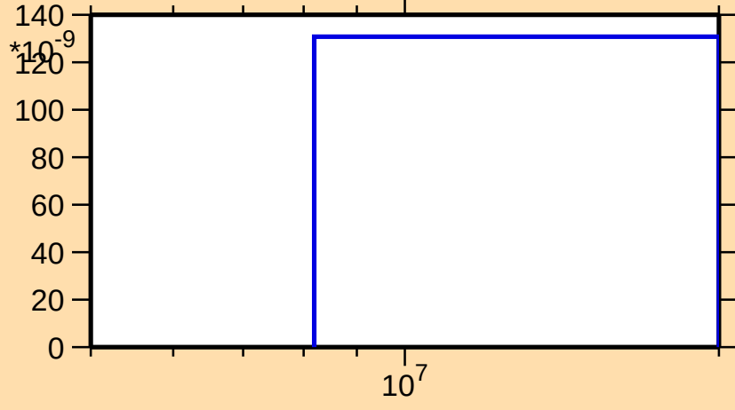
\sigma vs. E for ^{138}\text{Nd}(n,3n)
