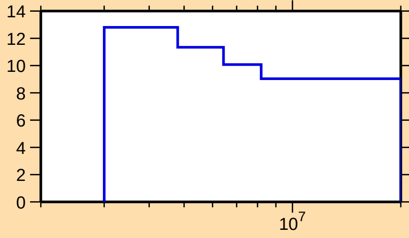
\Delta\sigma/\sigma vs. E for ^{138}\text{Nd}(n,n\text{onel.})
