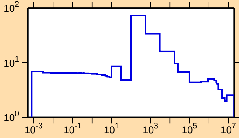
\sigma vs. E for ^{138}\text{Nd}(n,\text{el.})
