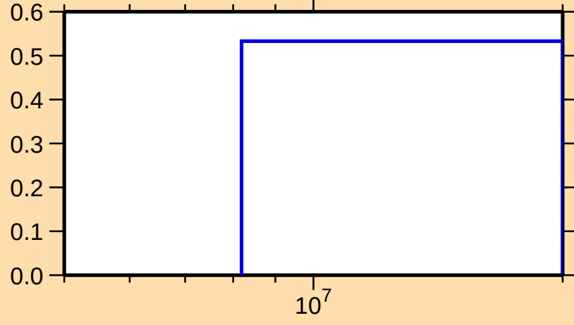
\sigma vs. E for ^{138}\text{Nd}(n,2n)
