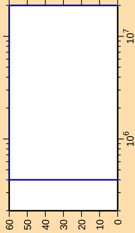
\Delta\sigma/\sigma vs. E for ^{138}\text{Nd}(n,\alpha)
