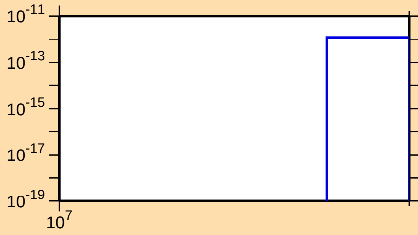
\sigma vs. E for ^{140}\text{Nd}(n,\text{nt})
