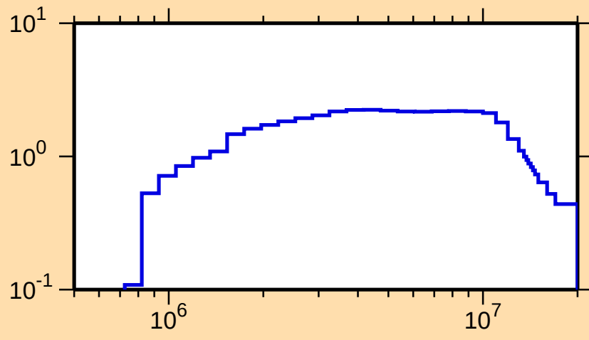
\sigma vs. E for ^{140}\text{Nd}(n,\text{inel.})
