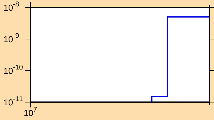
\sigma vs. E for ^{140}\text{Nd}(n,2n\alpha)
