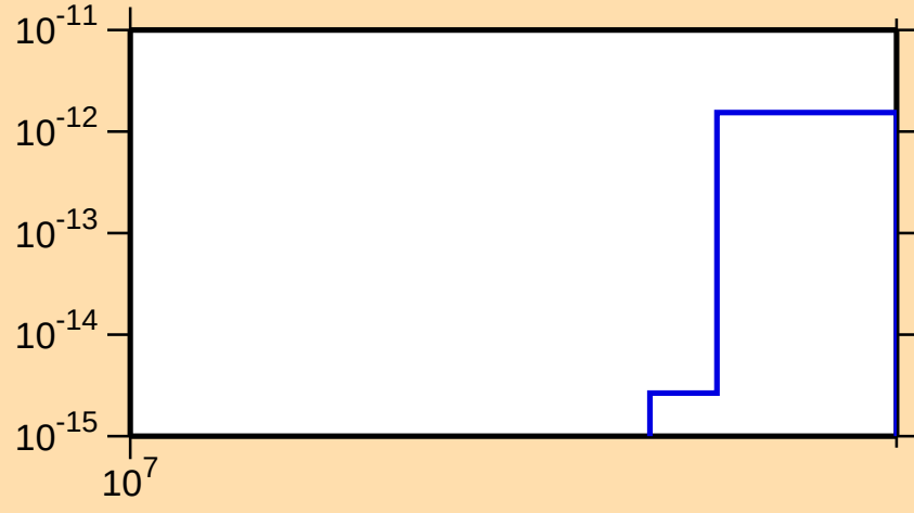
\sigma vs. E for ^{140}\text{Nd}(\text{mt } 45)
