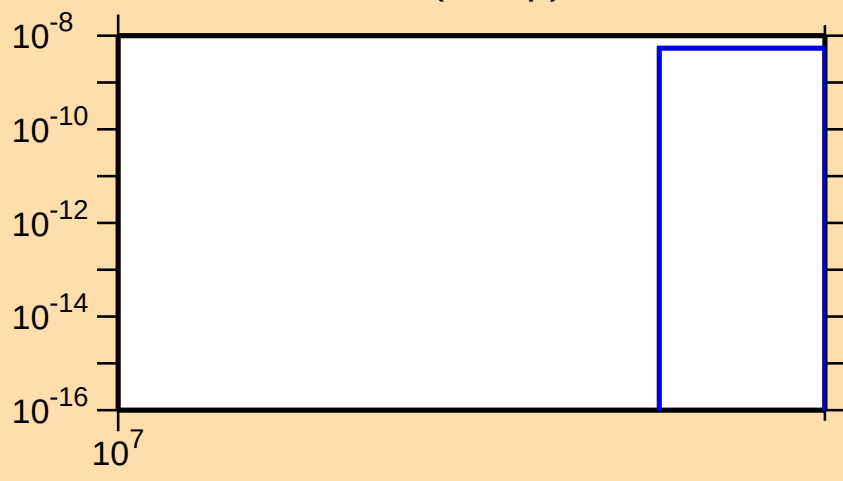
\sigma vs. E for ^{140}\text{Nd}(n,2np)
