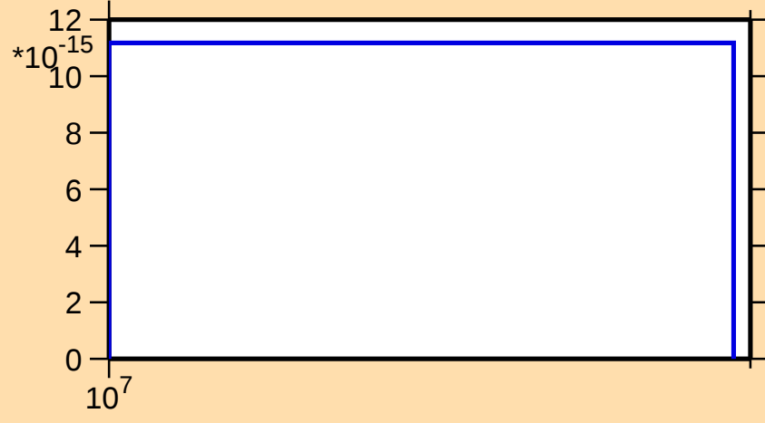
\sigma vs. E for ^{140}\text{Nd} (mt 45)
