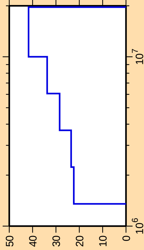
\Delta\sigma/\sigma vs. E for ^{140}\text{Nd}(n,n_3)
