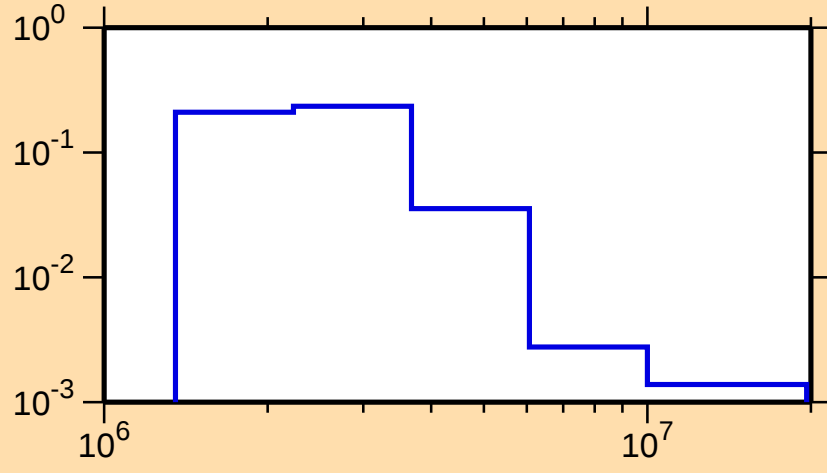
\sigma vs. E for ^{140}\text{Nd}(n,n_3)
