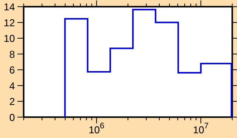
\Delta\sigma/\sigma vs. E for ^{140}\text{Nd}(n,\text{el.})
