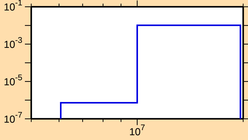
\sigma vs. E for ^{140}\text{Nd}(n,np)
