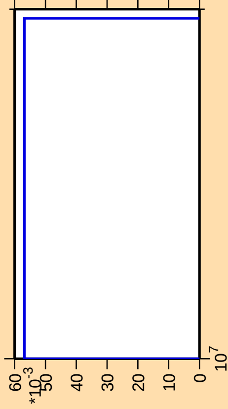
\Delta\sigma/\sigma vs. E for ^{140}\text{Nd} (mt 45)
