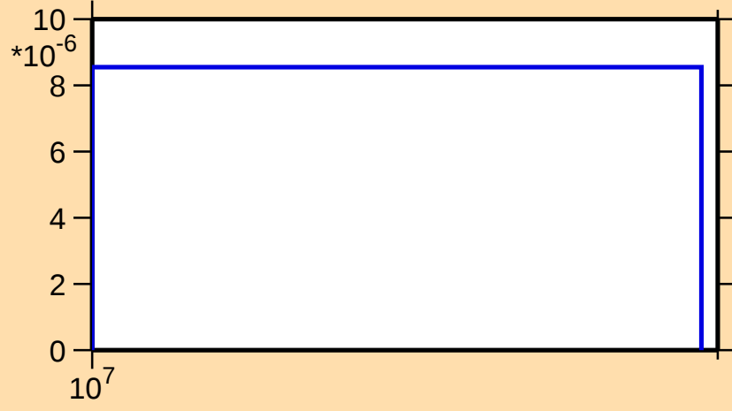
\sigma vs. E for ^{140}\text{Nd}(n,t)
