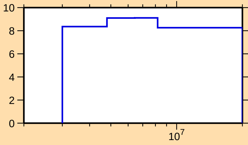
\Delta\sigma/\sigma vs. E for ^{140}\text{Nd}(n,n\text{onel.})
