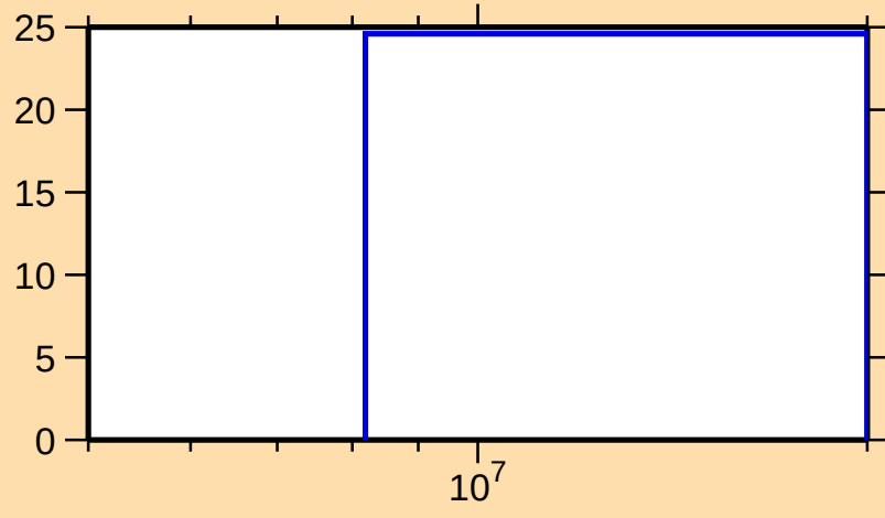
\Delta\sigma/\sigma vs. E for ^{140}\text{Nd}(n,\text{inel.})
