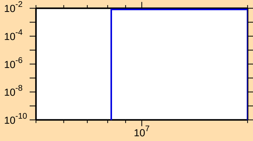
\sigma vs. E for ^{140}\text{Nd}(n,np)
