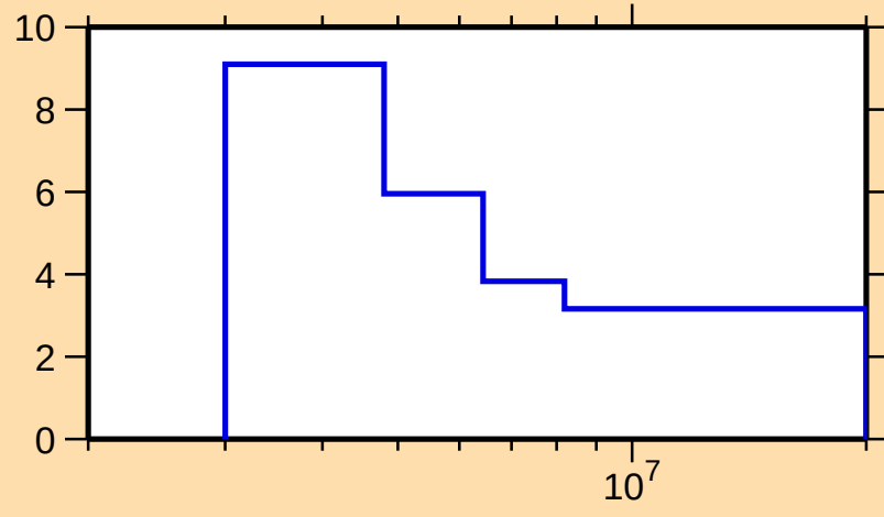
\Delta\sigma/\sigma vs. E for ^{140}\text{Nd}(n,\text{tot.})
