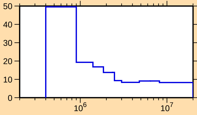
\Delta\sigma/\sigma vs. E for ^{140}\text{Nd}(n,\text{nonel.})
