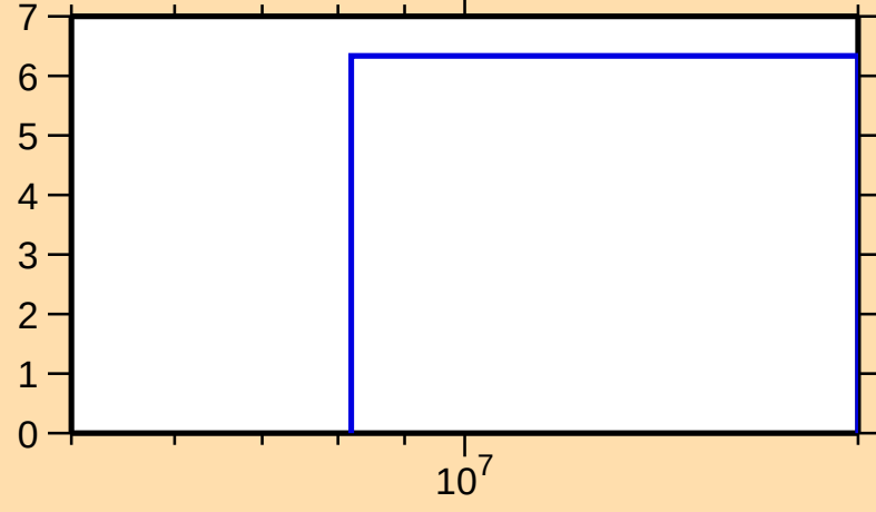
\Delta\sigma/\sigma vs. E for ^{140}\text{Nd}(n,\text{el.})
