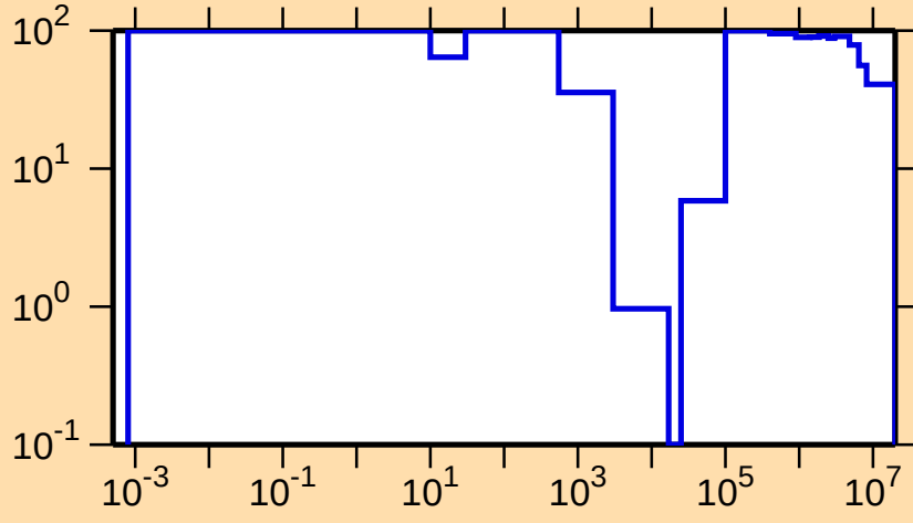
\Delta\sigma/\sigma vs. E for ^{140}\text{Nd}(n,p)
