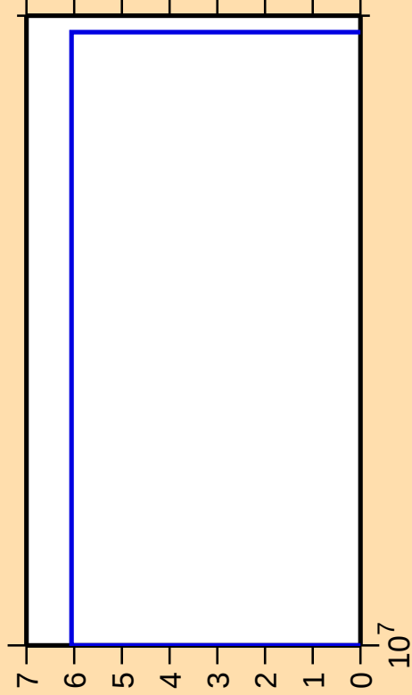
\Delta\sigma/\sigma vs. E for ^{141}\text{Nd}(n,\text{pd})
