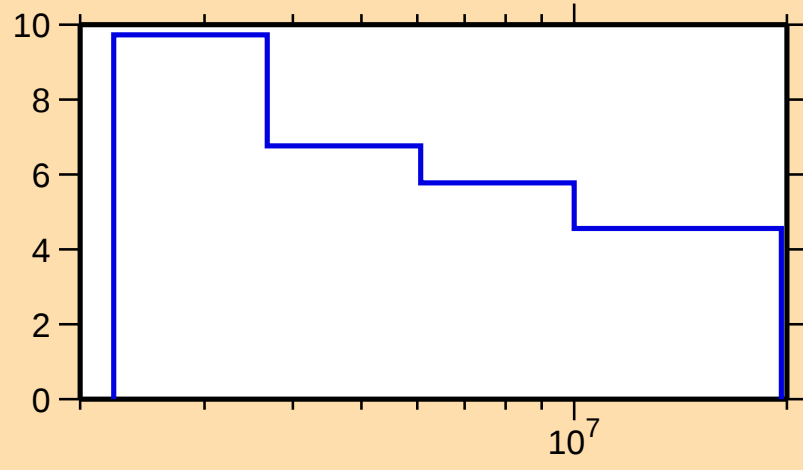
\Delta\sigma/\sigma vs. E for ^{141}\text{Nd}(n,n\text{onel.})
