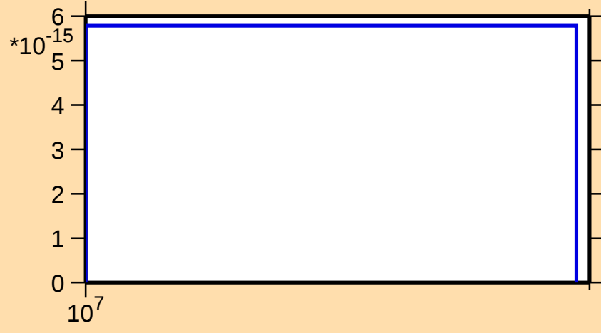
\sigma vs. E for ^{141}\text{Nd}(n,\text{nt})
