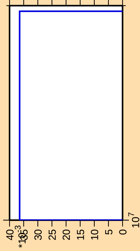
\Delta\sigma/\sigma vs. E for ^{141}\text{Nd}(n,\text{nt})
