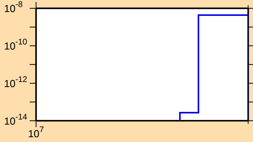
\sigma vs. E for ^{143}\text{Nd}(n,\text{nt})
