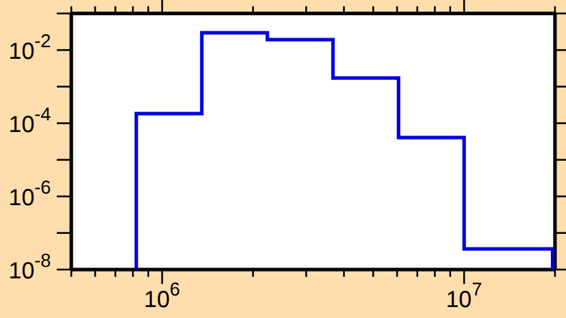
\sigma vs. E for ^{143}\text{Nd}(n,n_3)
