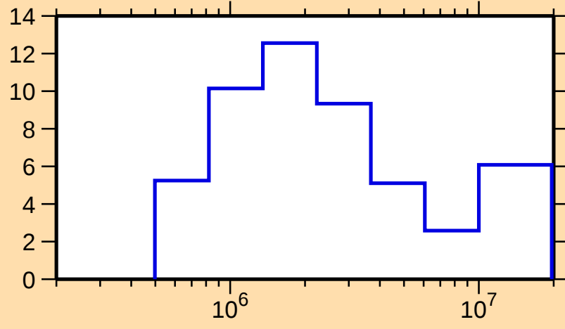
\Delta\sigma/\sigma vs. E for ^{143}\text{Nd}(n,\text{tot.})
