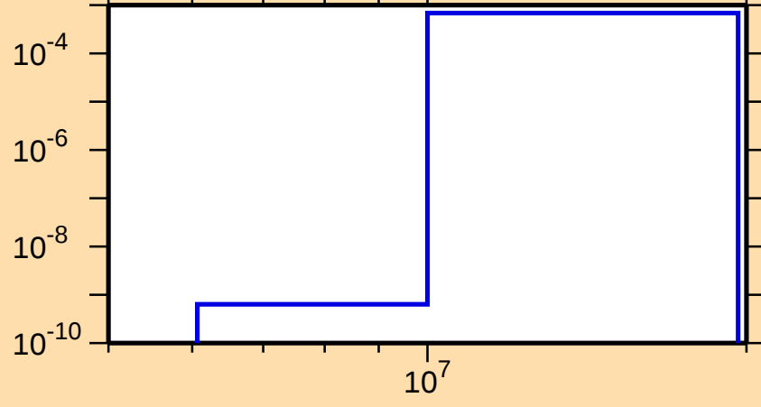
\sigma vs. E for ^{143}\text{Nd}(n,d)
