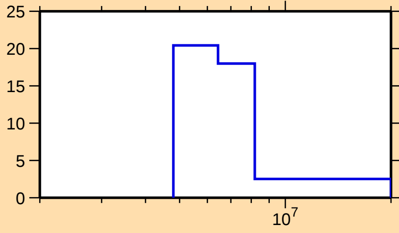
\Delta\sigma/\sigma vs. E for ^{143}\text{Nd}(n,2n)
