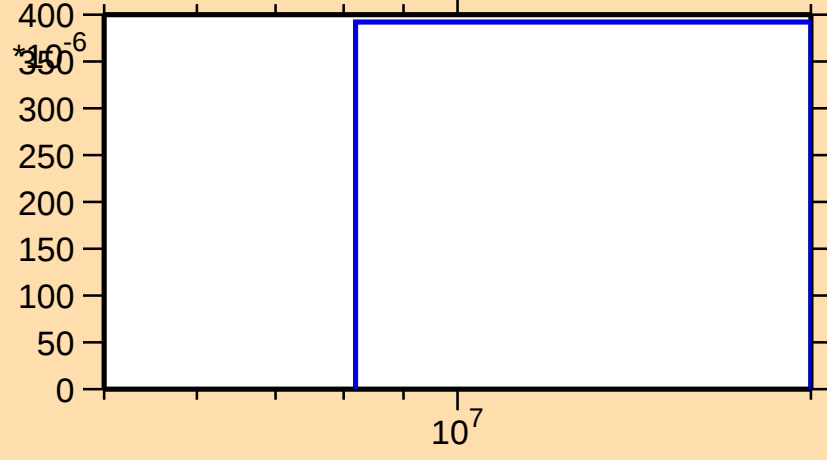
\sigma vs. E for ^{143}\text{Nd}(n,3n)
