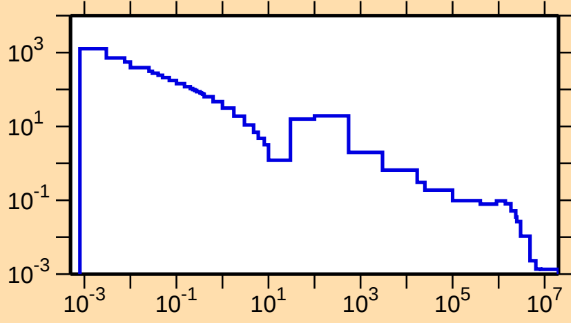
\sigma vs. E for ^{143}\text{Nd}(n,\gamma)
