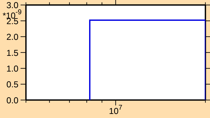
\sigma vs. E for ^{143}\text{Nd}(n,2n\alpha)
