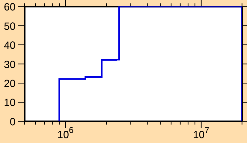
\Delta\sigma/\sigma vs. E for ^{143}\text{Nd}(n,\gamma)
