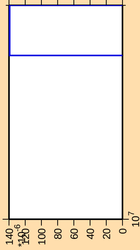
\Delta\sigma/\sigma vs. E for ^{144}\text{Nd}(\text{mt } 11)
