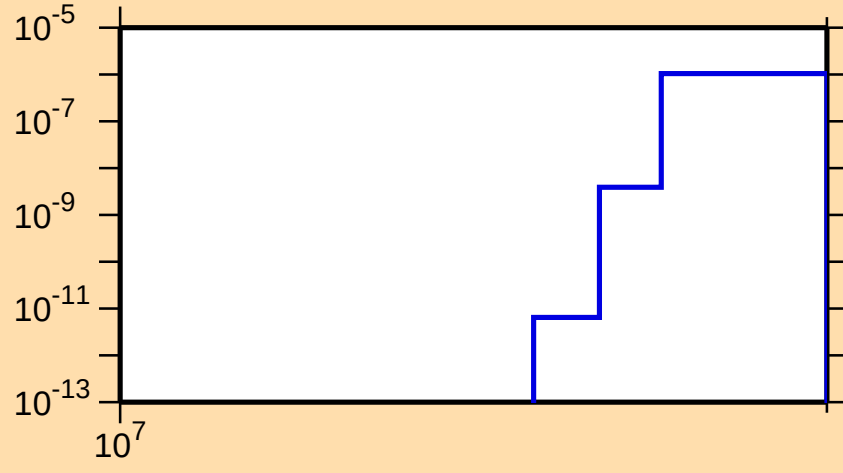
\sigma vs. E for ^{144}\text{Nd}(n,\text{nd})
