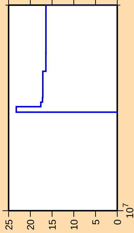
\Delta\sigma/\sigma vs. E for ^{144}\text{Nd}(n,3n)
