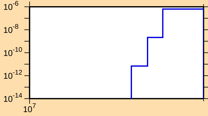
\sigma vs. E for ^{144}\text{Nd}(n,\text{nt})
