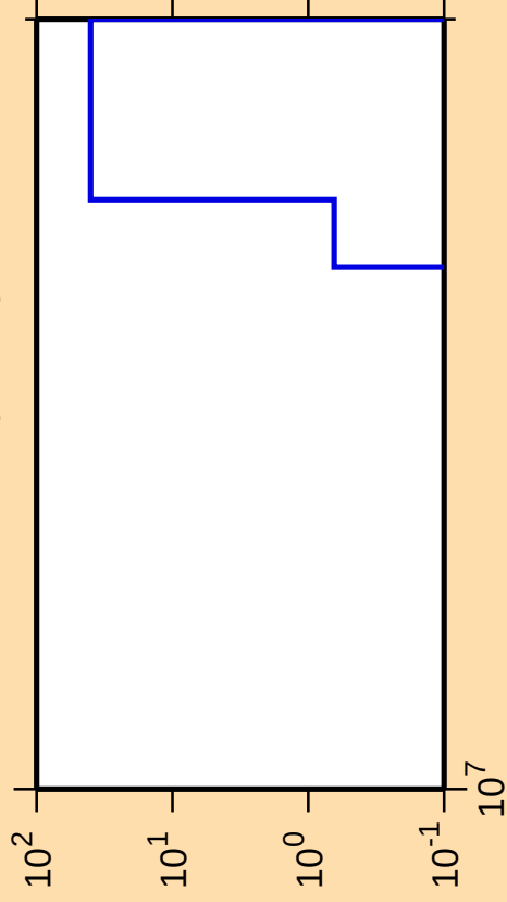
\Delta\sigma/\sigma vs. E for ^{144}\text{Nd} (mt 45)
