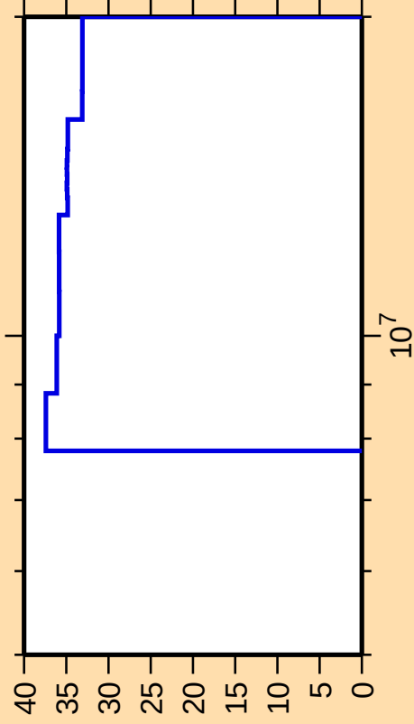
\Delta\sigma/\sigma vs. E for ^{144}\text{Nd}(n,n_1)
