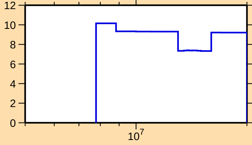
\Delta\sigma/\sigma vs. E for ^{144}\text{Nd}(n,2n)
