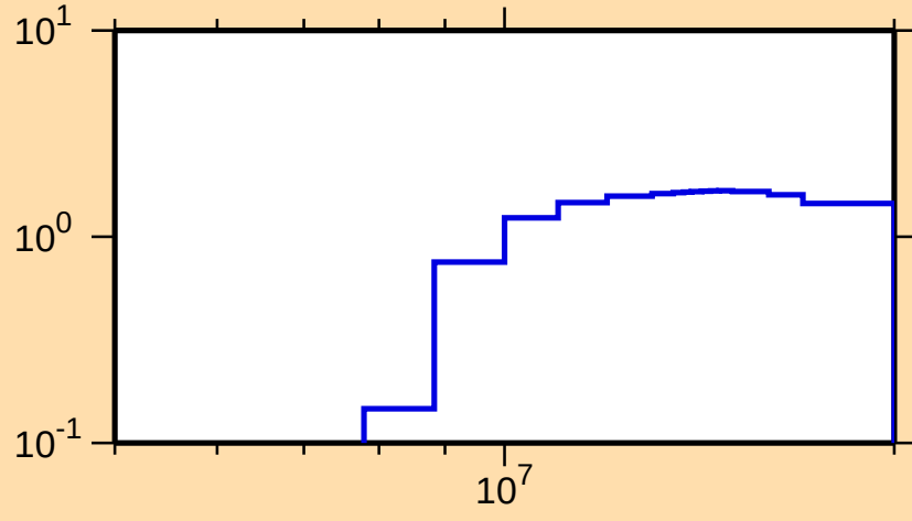
\sigma vs. E for ^{144}\text{Nd}(n,2n)
