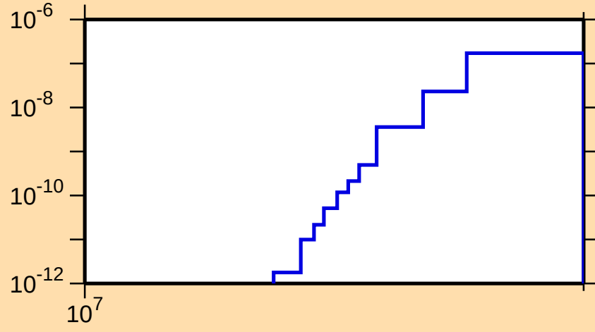
\sigma vs. E for ^{144}\text{Nd}(n,2n\alpha)
