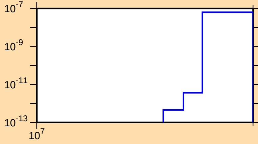
\sigma vs. E for ^{144}\text{Nd}(n,2np)
