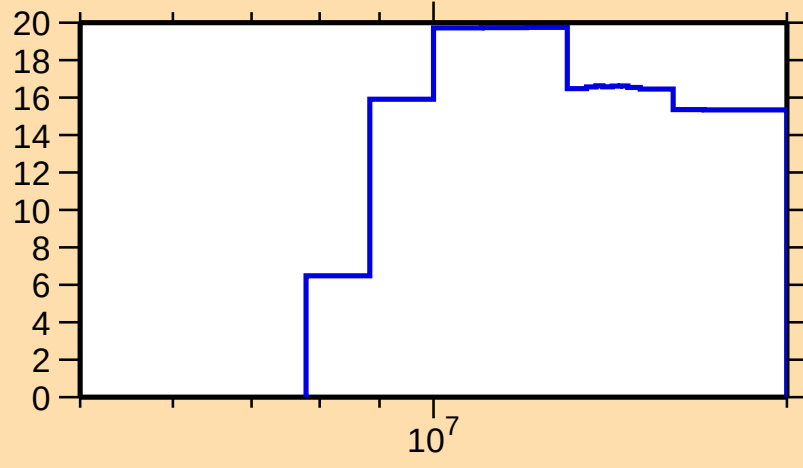
\Delta\sigma/\sigma vs. E for ^{144}\text{Nd}(n,\text{inel.})
