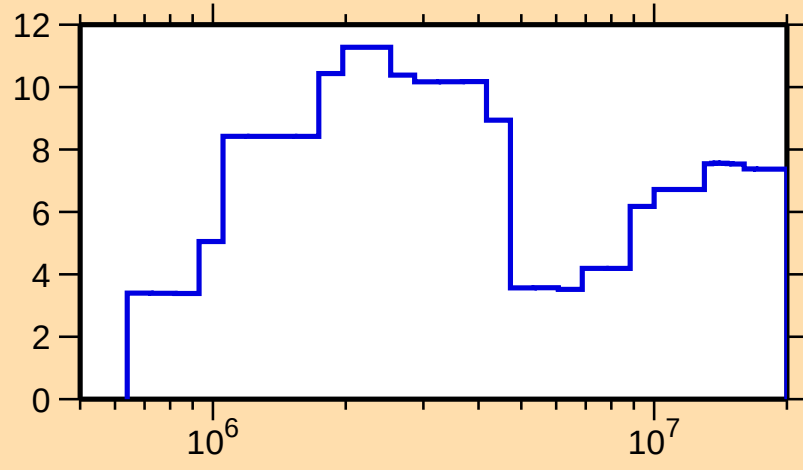
\Delta\sigma/\sigma vs. E for ^{144}\text{Nd}(n,\text{el.})
