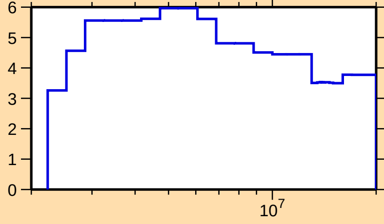
\Delta\sigma/\sigma vs. E for ^{144}\text{Nd}(n,\text{nonel.})
