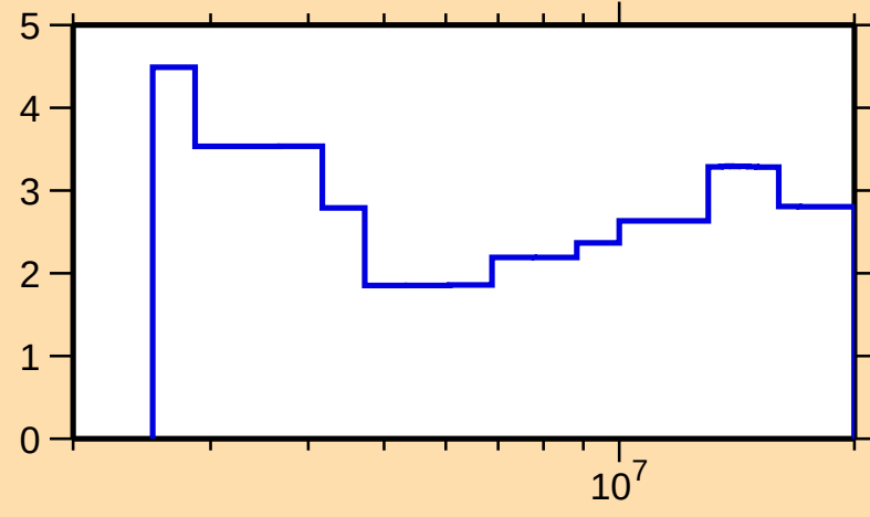
\Delta\sigma/\sigma vs. E for ^{144}\text{Nd}(n,\text{tot.})
