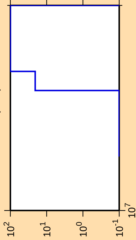
\Delta\sigma/\sigma vs. E for ^{144}\text{Nd}(n,\text{nt})
