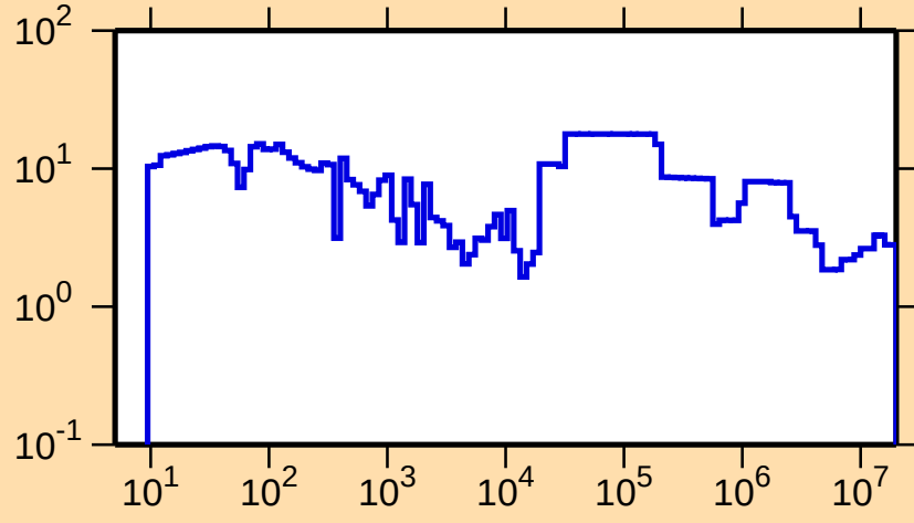
\Delta\sigma/\sigma vs. E for ^{144}\text{Nd}(n,\text{tot.})
