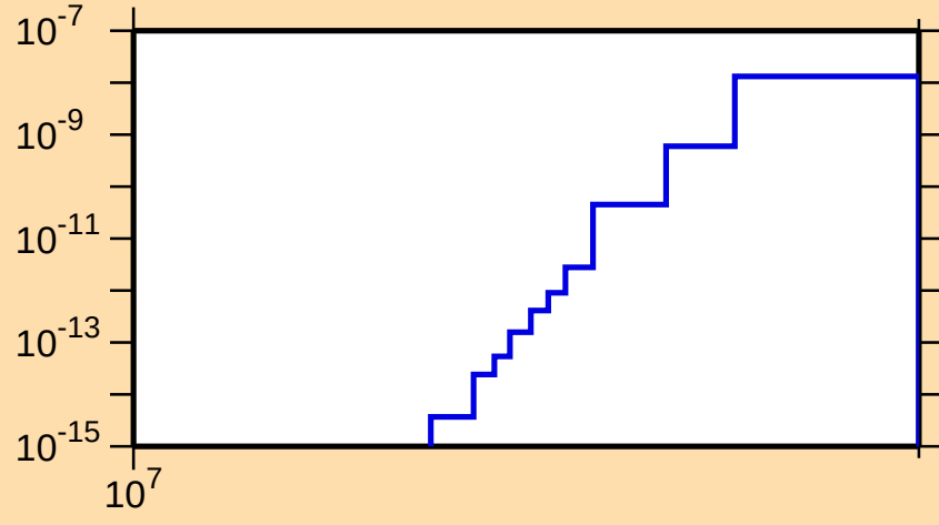
\sigma vs. E for ^{144}\text{Nd}(n,\text{He3})
