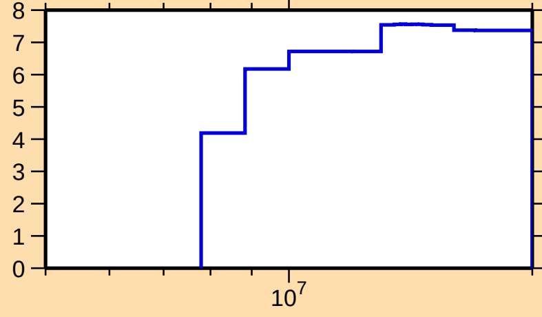
\Delta\sigma/\sigma vs. E for ^{144}\text{Nd}(n,\text{el.})
