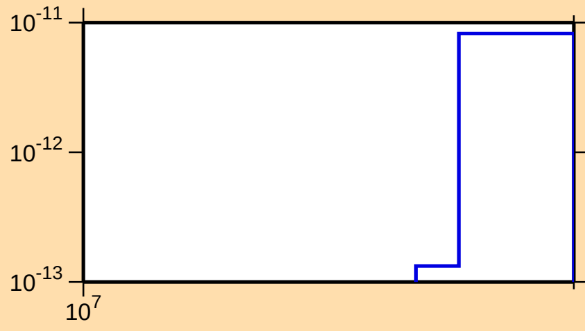
\sigma vs. E for ^{144}\text{Nd} (mt 45)
