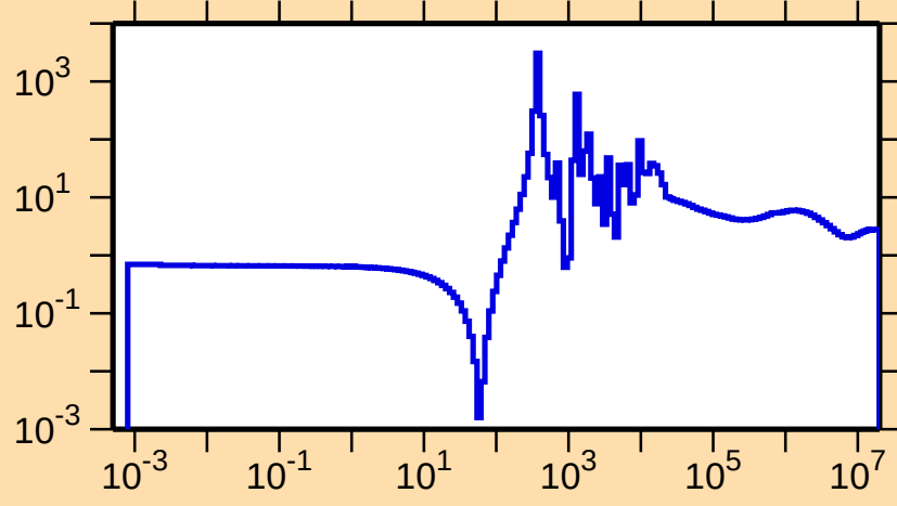
\sigma vs. E for ^{144}\text{Nd}(n,\text{el.})
