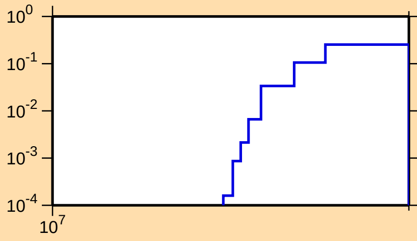
\sigma vs. E for ^{144}\text{Nd}(n,3n)
