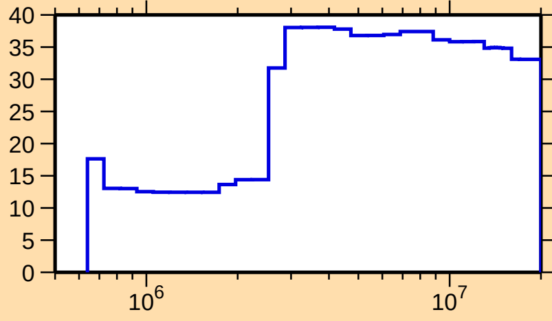
\Delta\sigma/\sigma vs. E for ^{144}\text{Nd}(n,n_1)
