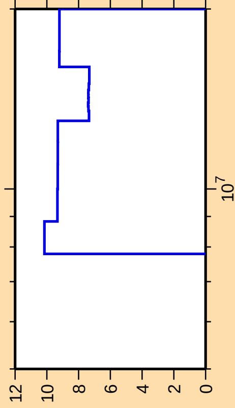
\Delta\sigma/\sigma vs. E for ^{144}\text{Nd}(n,2n)
