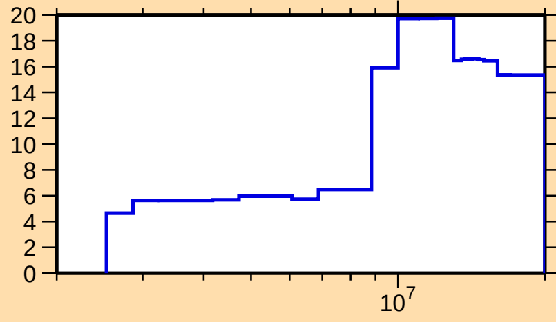
\Delta\sigma/\sigma vs. E for ^{144}\text{Nd}(n,\text{inel.})
