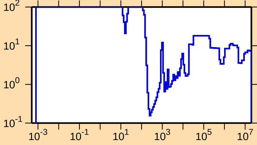
\Delta\sigma/\sigma vs. E for ^{144}\text{Nd}(n,\text{el.})
