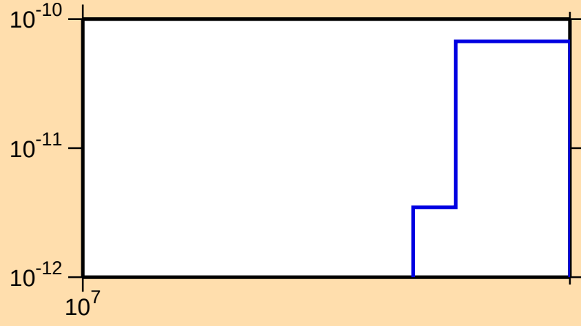
\sigma vs. E for ^{144}\text{Nd}(\text{mt117})
