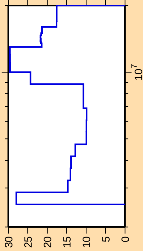
\Delta\sigma/\sigma vs. E for ^{144}\text{Nd}(n,n_{\text{cont}}) .
