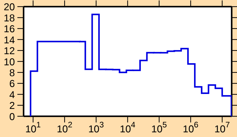
\Delta\sigma/\sigma vs. E for ^{144}\text{Nd}(n,\text{nonel.})
