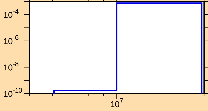
\sigma vs. E for ^{144}\text{Nd}(n,d)
