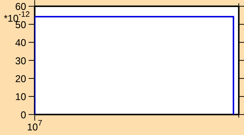
\sigma vs. E for ^{144}\text{Nd}(n,p\alpha)
