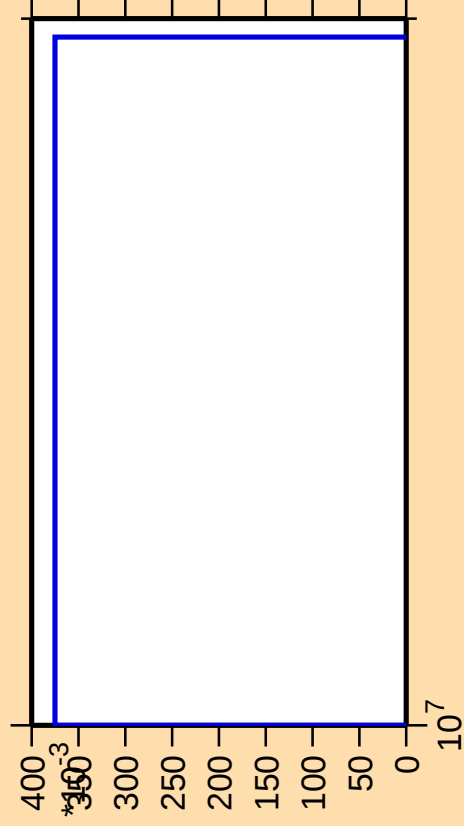
\Delta\sigma/\sigma vs. E for ^{144}\text{Nd}(\text{mt } 45)
