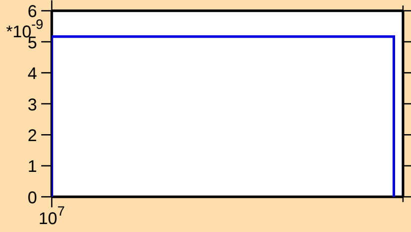
\sigma vs. E for ^{144}\text{Nd}(n,\text{nt})
