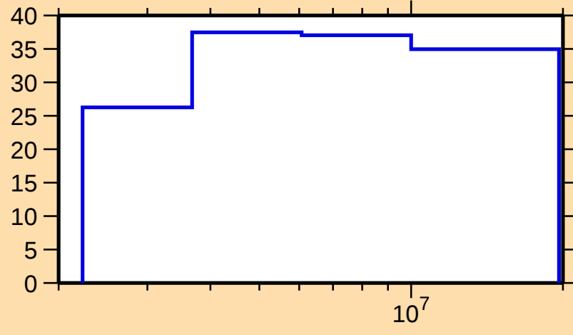
\Delta\sigma/\sigma vs. E for ^{144}\text{Nd}(n,n_1)
