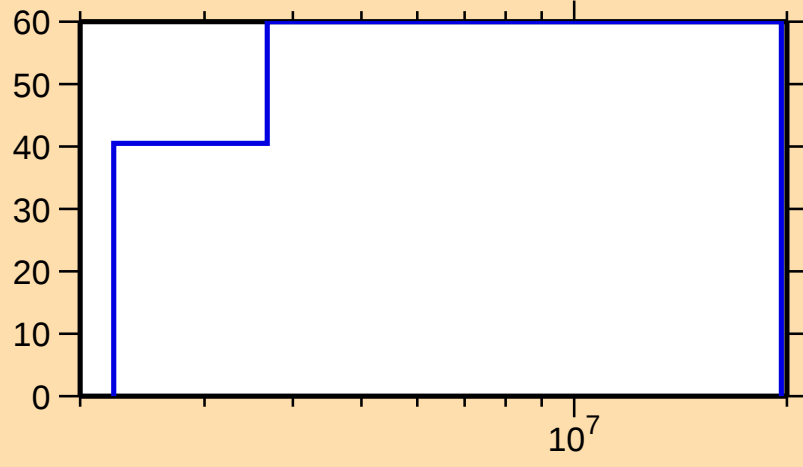
\Delta\sigma/\sigma vs. E for ^{144}\text{Nd}(n,\gamma)
