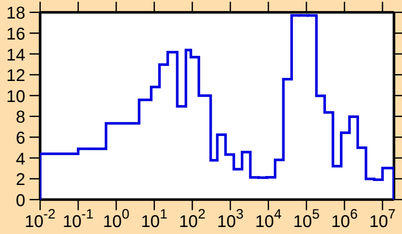
\Delta\sigma/\sigma vs. E for ^{144}\text{Nd}(n,\text{tot.})
