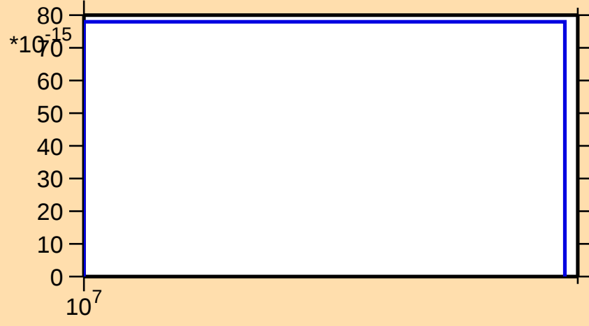
\sigma vs. E for ^{144}\text{Nd}(\text{mt } 45)
