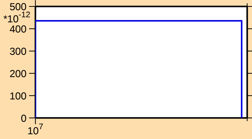
\sigma vs. E for ^{144}\text{Nd}(n,2np)
