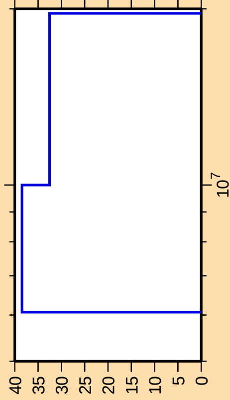
\Delta\sigma/\sigma vs. E for ^{144}\text{Nd}(n,\alpha)
