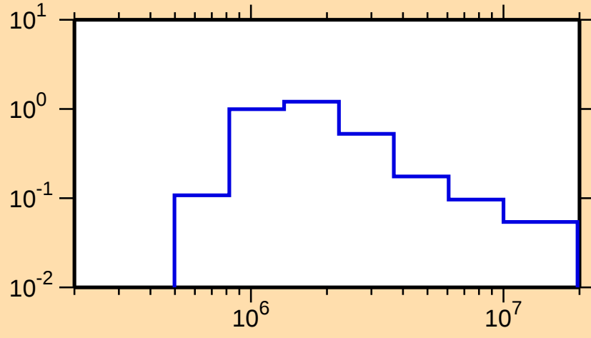
\sigma vs. E for ^{144}\text{Nd}(n,n_1)
