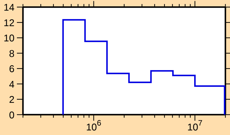
\Delta\sigma/\sigma vs. E for ^{144}\text{Nd}(n,\text{nonel.})
