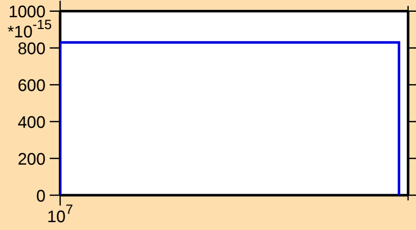
\sigma vs. E for ^{144}\text{Nd}(\text{mt117})
