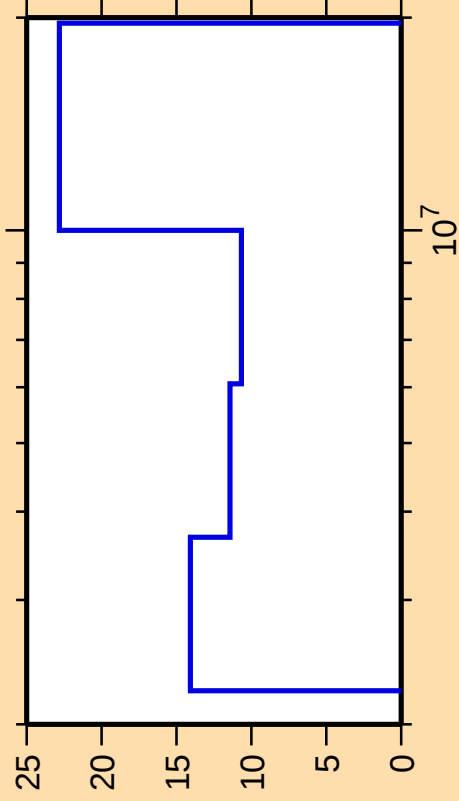
\Delta\sigma/\sigma vs. E for ^{144}\text{Nd}(n,\text{ncont.})
