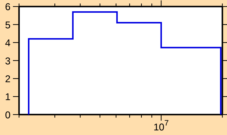
\Delta\sigma/\sigma vs. E for ^{144}\text{Nd}(n,n\text{onel.})
