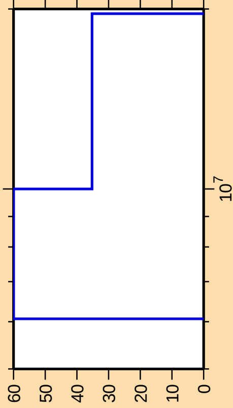
\Delta\sigma/\sigma vs. E for ^{144}\text{Nd}(n,p)
