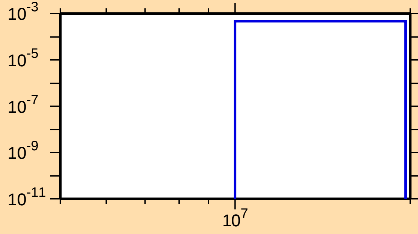
\sigma vs. E for ^{144}\text{Nd}(n,np)
