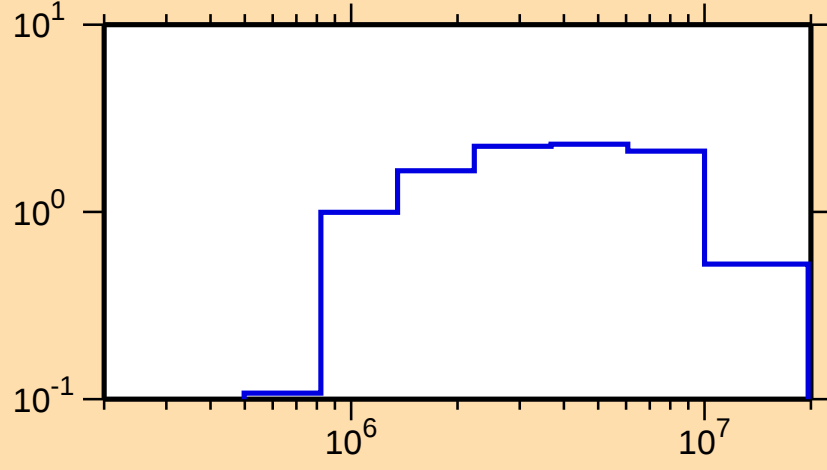
\sigma vs. E for ^{144}\text{Nd}(n,\text{inel.})
