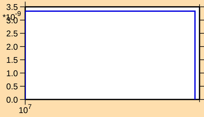
\sigma vs. E for ^{144}\text{Nd}(n,2n\alpha)
