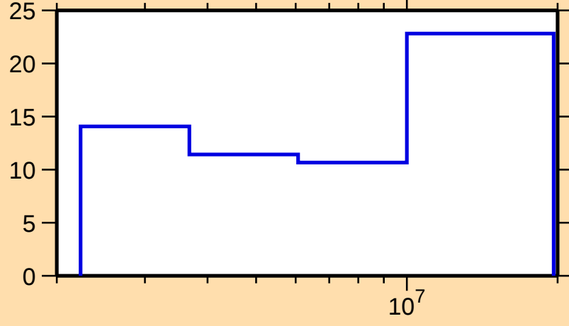
\Delta\sigma/\sigma vs. E for ^{144}\text{Nd}(n,n\text{cont.})
