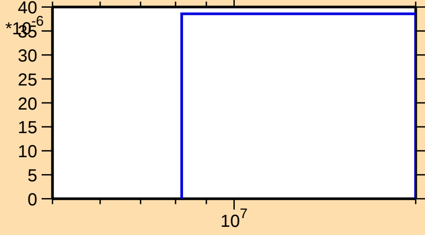
\sigma vs. E for ^{144}\text{Nd}(n,t)
