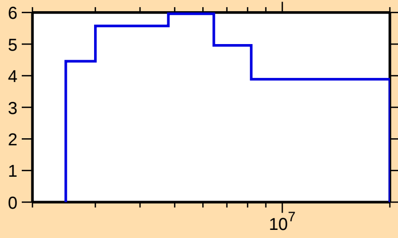
\Delta\sigma/\sigma vs. E for ^{144}\text{Nd}(n,n\text{nonel.})
