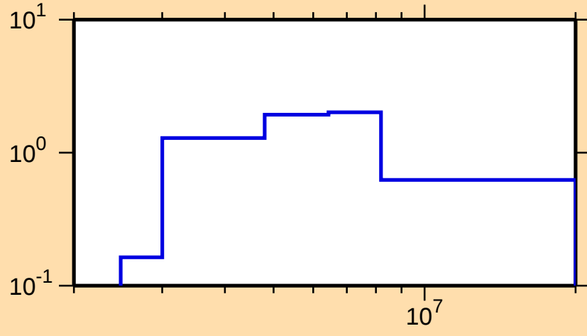
\sigma vs. E for ^{144}\text{Nd}(n,n\text{cont.})
