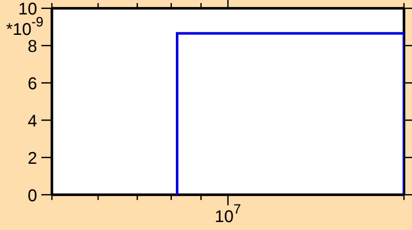
\sigma vs. E for ^{144}\text{Nd}(n,\text{nd})
