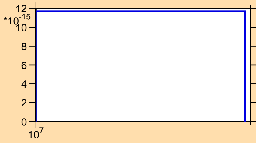
\sigma vs. E for ^{149}\text{Nd}(n,\text{He}3)
