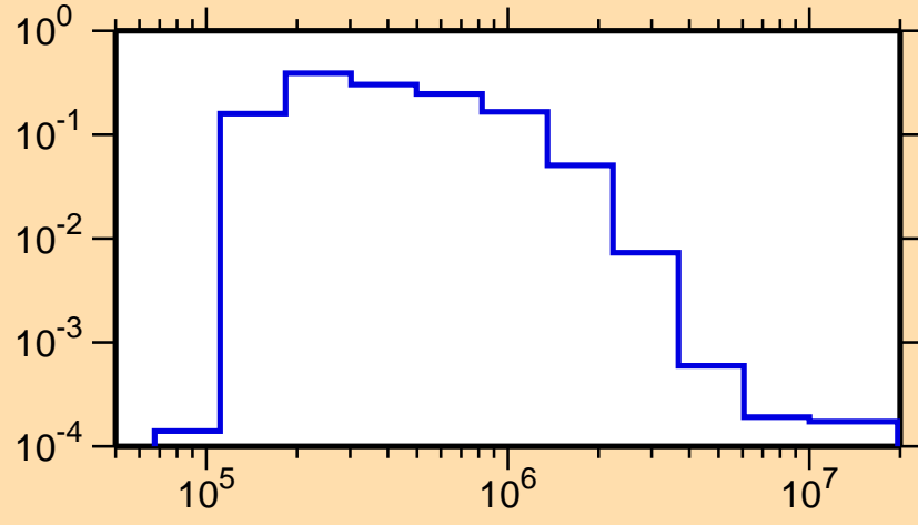
\sigma vs. E for ^{149}\text{Nd}(n,n_1)
