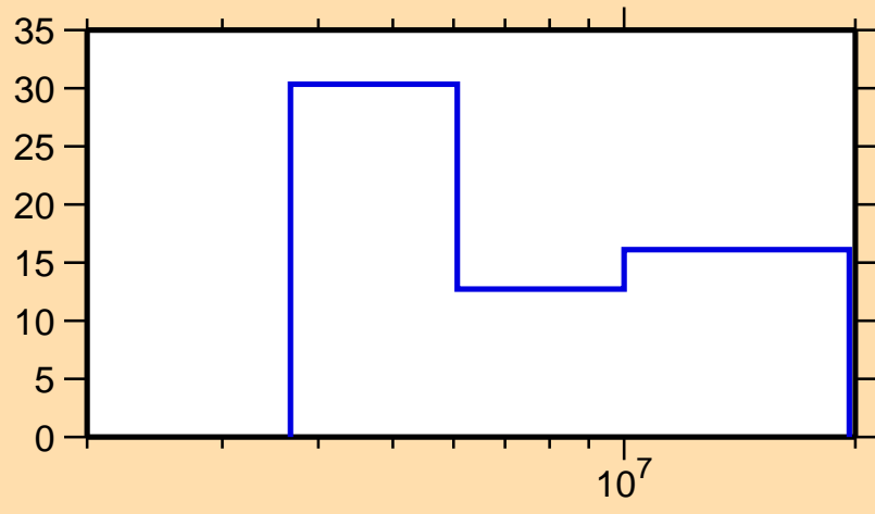
\Delta\sigma/\sigma vs. E for ^{149}\text{Nd}(n,2n)
