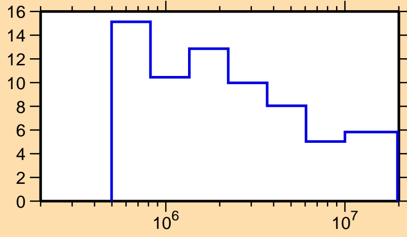
\Delta\sigma/\sigma vs. E for ^{149}\text{Nd}(n,\text{tot.})
