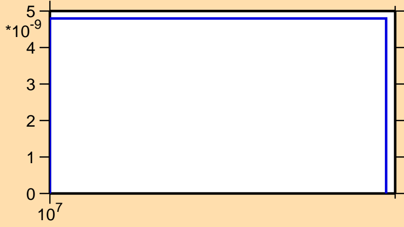
\sigma vs. E for ^{149}\text{Nd}(n,nt)
