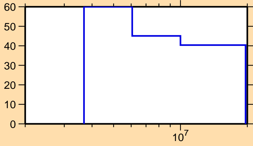
\Delta\sigma/\sigma vs. E for ^{149}\text{Nd}(n,p)
