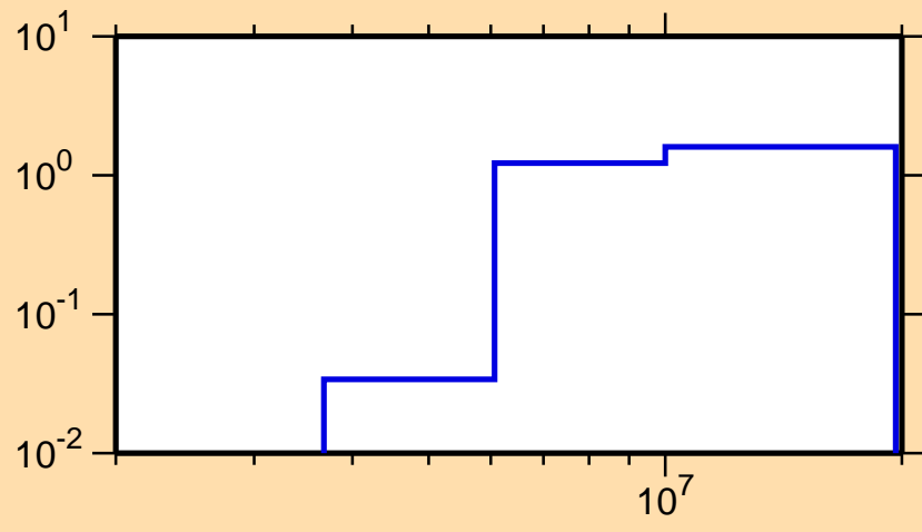
\sigma vs. E for ^{149}\text{Nd}(n,2n)
