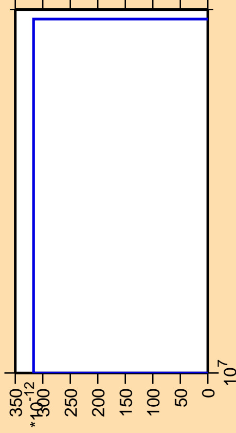
\Delta\sigma/\sigma vs. E for ^{149}\text{Nd} (mt 11)
