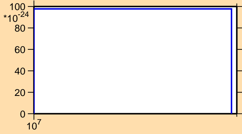
\sigma vs. E for ^{149}\text{Nd} (mt 11)
