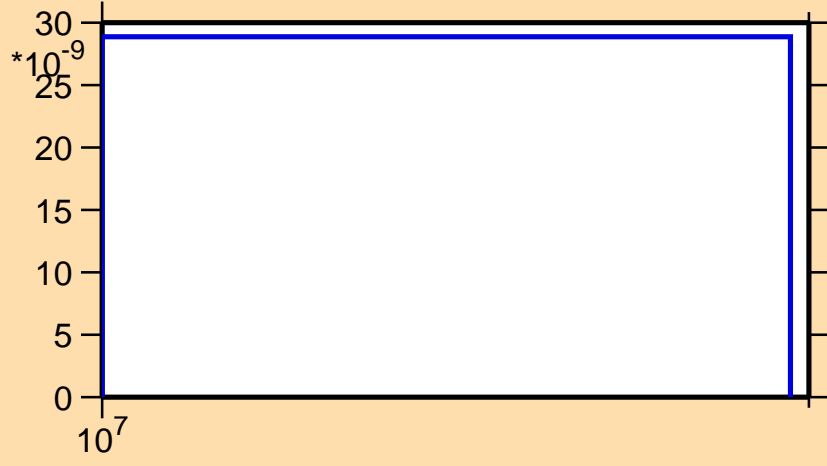
\sigma vs. E for ^{149}\text{Nd}(n,\text{nd})
